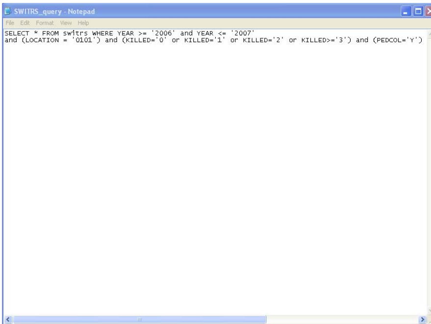
Figure E 6. Query displayed in Notepad
