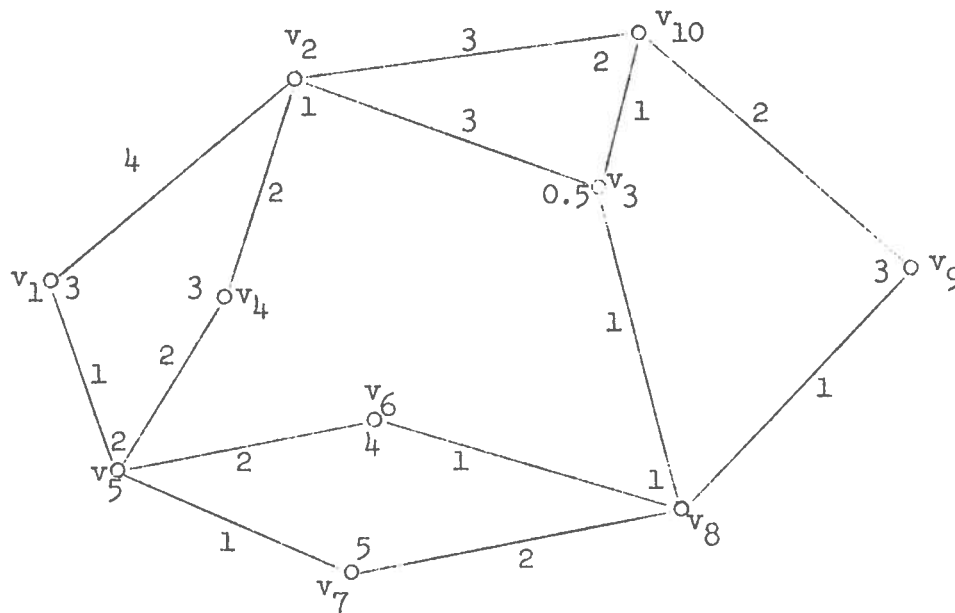
Figure 1: An Example Weighted Graph
