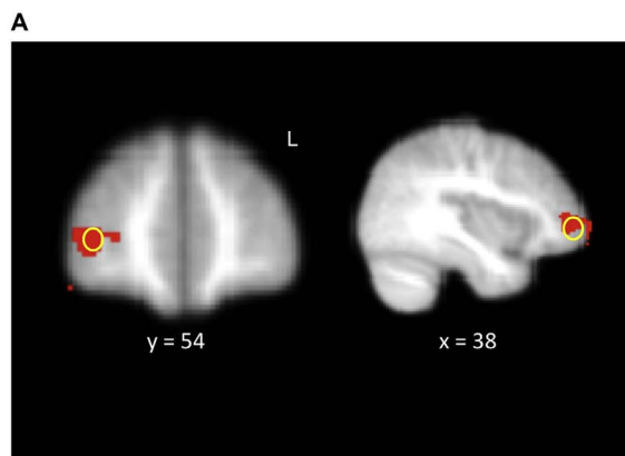
Fig. 5. (A) Stress \times Age \times Gender interaction in the right frontal pole ( x=38 , y=54 , z=4 ) for ADV Risk > DIS Risk contrast. (B) Adolescent males showed a decrease in right frontal pole activation from low stress to high stress when taking ADV Risk > DIS Risk while adult males showed a trend towards an increase in right frontal pole activation from low stress to high stress when taking ADV Risk > DIS Risk.
