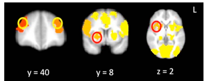
Fig. 6. For ADV Risk > DIS Risk contrast, averaged across stress, age and gender, mean activation was found in bilateral frontal pole (left: x=-40 , y=40 , z=30 , right: x=50 , y=42 , z=18 ), right putamen ( x=24 , y=8 , z=4 ), and right anterior insula ( x=38 , y=16 , z=2 ).
