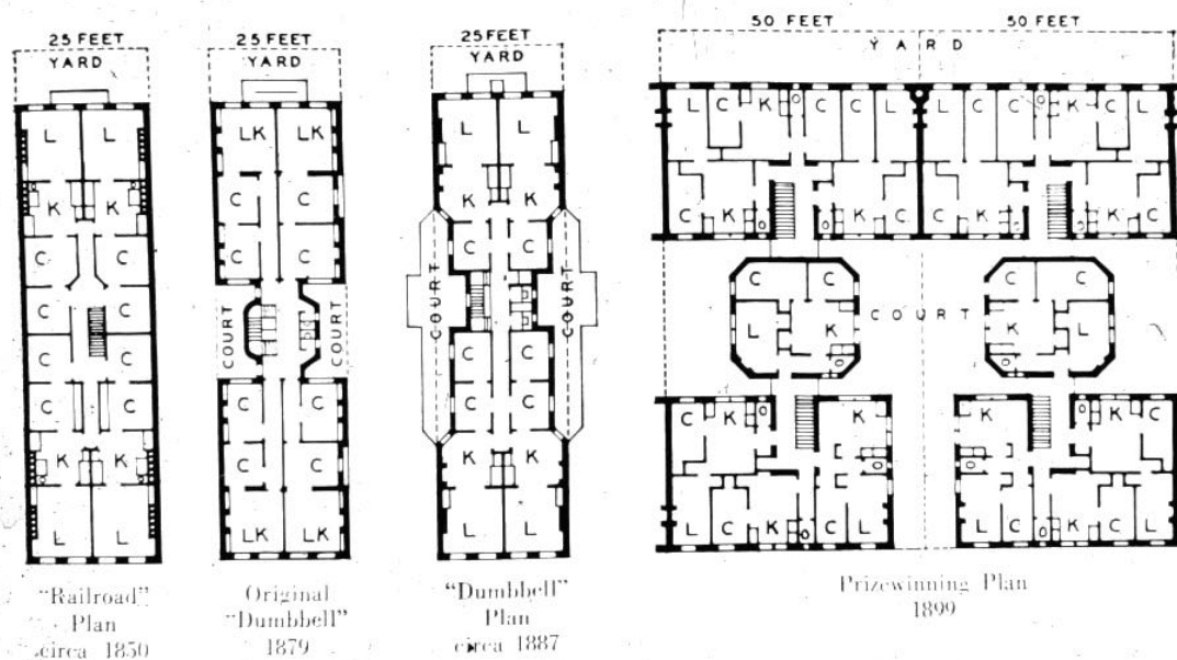
Figure 4.3: Evolution of a typical New York City tenement building, 1850-1900. Letters indicate chambers/bedrooms (C), living rooms/parlors (L), and kitchens (K). Sources: New York Public Library, Columbia University.
