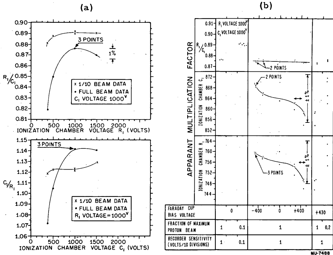
Fig. 26. Results of calibration of a \parallel -plate ionization chamber for (a) the saturation effect with beam intensity, (b) apparent multiplication factor with beam intensity and Faraday cup bias voltage.
