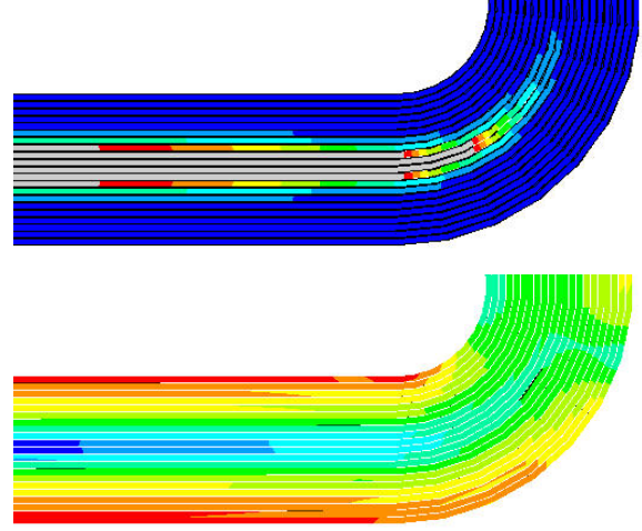
Fig. 15. A coil normal zone after 80 ms with T_{\max} = 44 K (top) and a local compressive stress of -136 MPa after 480 msec when the local temperature reaches 300 K (bottom).
