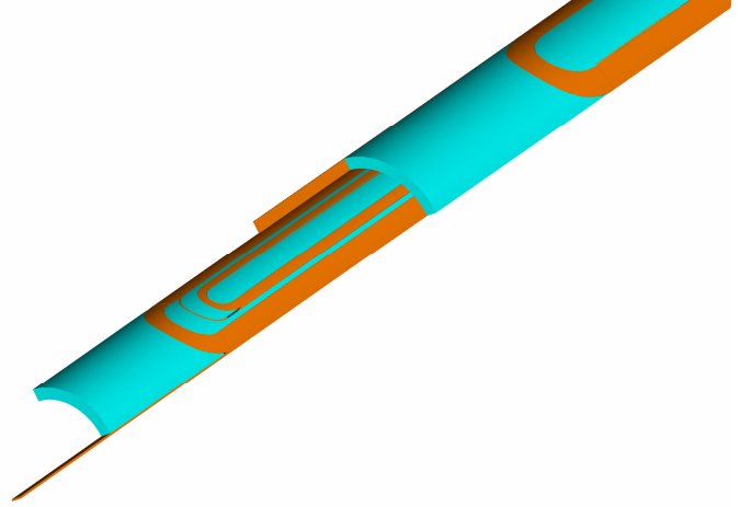
Fig. 3. Typical nesting coils and spacers in CAD ProE.
