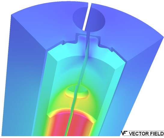
Fig. 5. Magnetic model details of optimized iron features above the coil ends.
