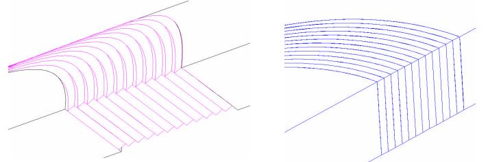
Fig. 7 Stacked coil edges around the ends (left) are extend to meet round smooth surfaces on both coils ID and OD (right)
