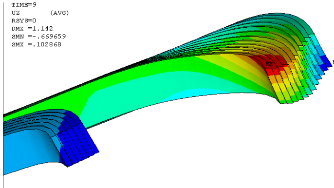
Fig. 10. A deformed coil end region under Lorentz forces modeled with friction between turns.
