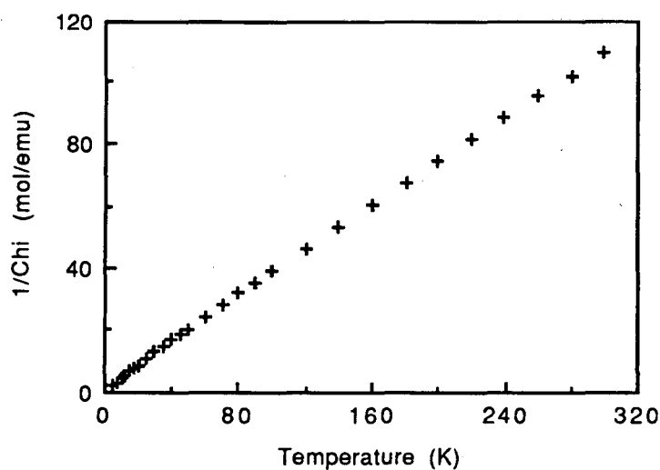
Figure 21. Plot of 1/\chi_M vs. T for [(\text{Me}_5\text{C}_5)_2\text{Yb}]_2(\mu\text{-BH}_4) .
