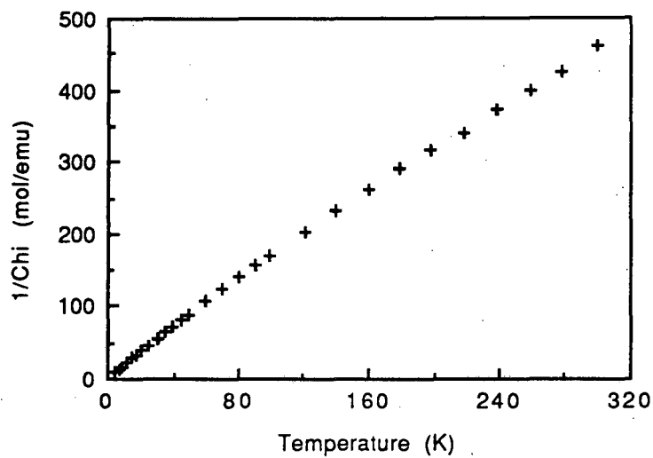
Figure 6. Plot of 1/\chi_M vs. T for (\text{Me}_5\text{C}_5)_2\text{Yb}(\mu\text{-H})\text{Ti}(\text{Me}_5\text{C}_5)_2 .
