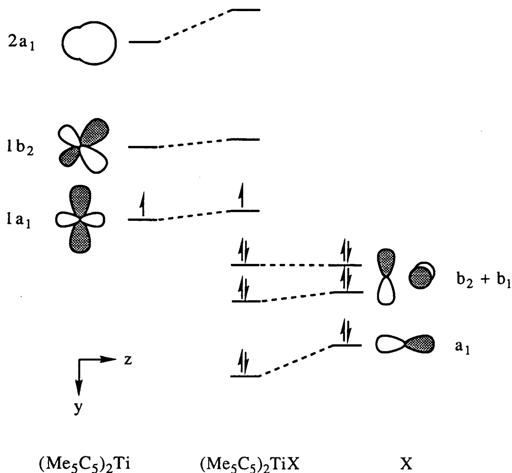
Figure 12. Molecular Orbital Diagram for (\text{Me}_5\text{C}_5)_2\text{TiX} , \text{C}_{2v} symmetry.
