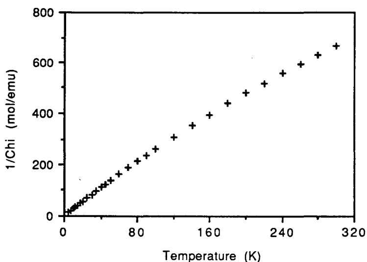
Figure 1. Plot of 1/\chi_M vs. T for (\text{Me}_5\text{C}_5)_2\text{TiH} .
