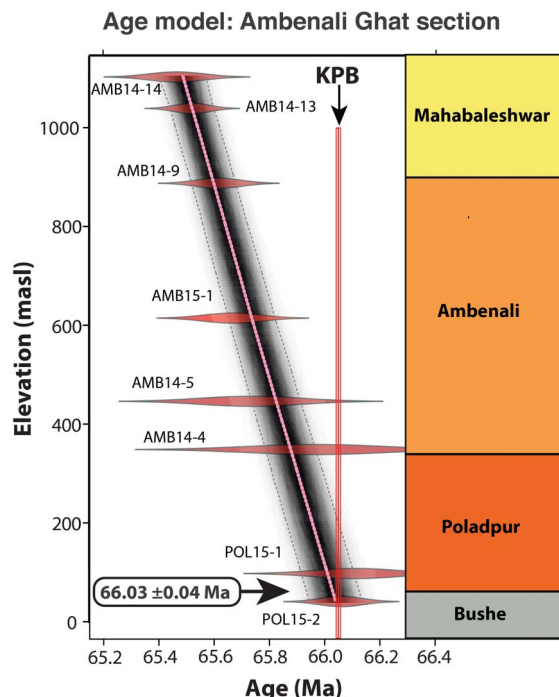
Fig. 3. Bayesian age model for the Ambenali Ghat section.
