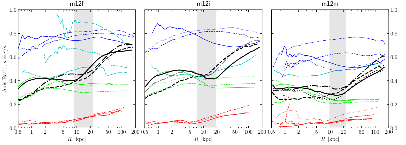
Figure B1. Shape profiles of simulated MW-mass galaxies as a function of R . Minor-to-major axis ratio s = c/a as a function of geometrical mean radius R for different species (DM, stars, and gas) in three sets of MW-mass galaxy simulations: m12f (left), m12i (centre), and m12m (right). Line-styles, colours, and shaded-areas follow the legend in Figure 4. An alternate version of this plot using the semi-major axis r = a can be found in the main body of the work in Figure 8. The literature often plots axis ratios versus this geometrical mean of the axis lengths R , which is therefore given here for comparison purposes. We note that the main difference is in how the curves have shifted leftward towards smaller radii.
