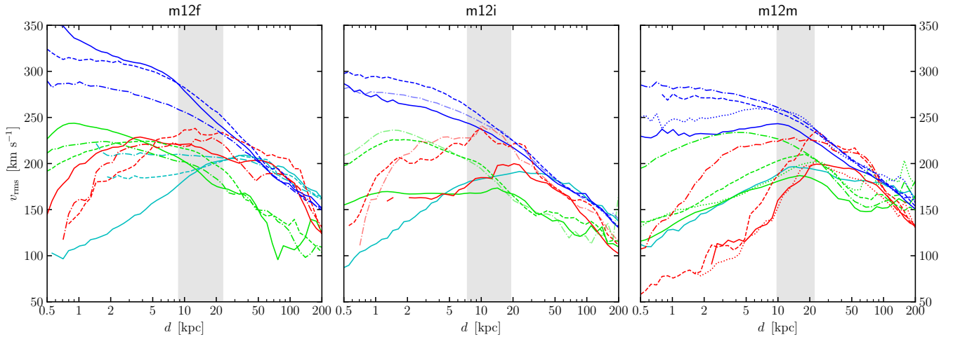
Figure 6. Ellipsoidally-averaged velocity profiles of the simulated MW-mass galaxies. Root-mean-square velocity v_{\text{rms}} as a function of ellipsoidal distance d for m12f (left), m12i (centre), and m12m (right). Line-styles, colours, and shaded-areas follow the legend in Figure 4.
