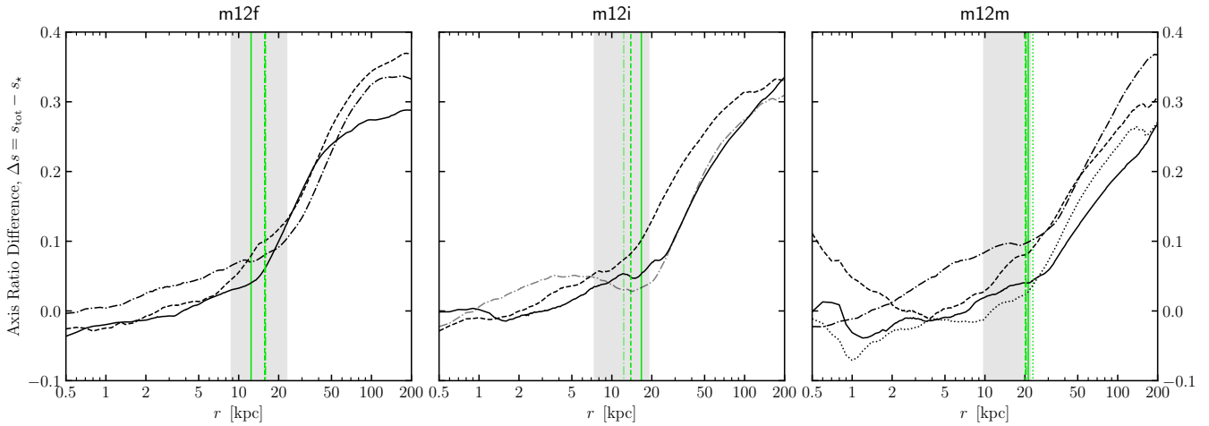
Figure 11. Difference in shape profiles of simulated MW-mass galaxies. Minor-to-major axis ratio difference \Delta s = s_{\text{tot}} - s_{\star} is shown as a function of semi-major axis r = a in three sets of MW-mass galaxy simulations: m12f (left), m12i (centre), and m12m (right). Line-styles and shaded-areas follow the legend in Figure 4. The black curves represent the axis ratio difference \Delta s and the vertical lines represent r_{\star,90} , the spherical radius of 90% of stellar mass within 30 kpc of the central galaxy, given in Table 1.
