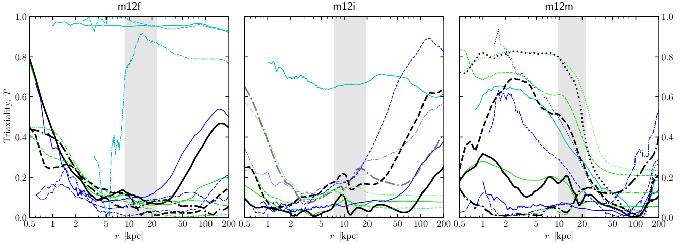
Figure 9. Triaxiality profiles of simulated MW-mass galaxies. Triaxiality T is shown as a function of semi-major axis r = a for different species (DM and stars) in three sets of MW-mass galaxy simulations: m12f (left), m12i (centre), and m12m (right). Line-styles, colours, and shaded-areas follow the legend in Figure 4. An alternate version of this plot using the geometrical mean of the axis lengths, R = (abc)^{1/3} , can be found in Appendix B.
