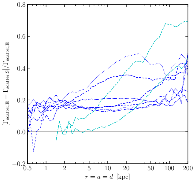
Figure A1. Difference in DM local collision rate of simulated MW-mass galaxies. The difference when averaging over shells of ellipsoidal distances d versus spherical radii r = a , [\Gamma_{\text{scatter,E}}(d) - \Gamma_{\text{scatter,S}}(r)] / \Gamma_{\text{scatter,E}}(d) (Equation 6) as a function of d = r = a for SIDM simulations. Shells are matched so that spherical radius r is equal to the semi-major axis a of the ellipsoid used to compute d . Line-styles and colours follow the legend in Figure 4. Using ellipsoidal shells leads to larger \Gamma_{\text{scatter}} , mostly because of an increase in the computed DM density. The difference in the local collision rate increases for the ellipsoidal shells method away from the centre of the galaxies.
