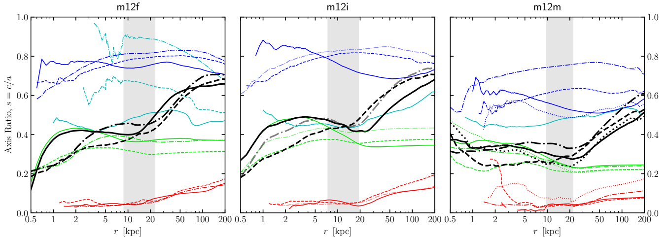
Figure 8. Shape profiles of simulated MW-mass galaxies. Minor-to-major axis ratio s = c/a is shown as a function of semi-major axis r = a for different species (DM, stars, and gas) in three sets of MW-mass galaxy simulations: m12f (left), m12i (centre), and m12m (right). Line-styles, colours, and shaded-areas follow the legend in Figure 4. An alternate version of this plot using the geometrical mean of the axis lengths, R = (abc)^{1/3} , can be found in Appendix B.
