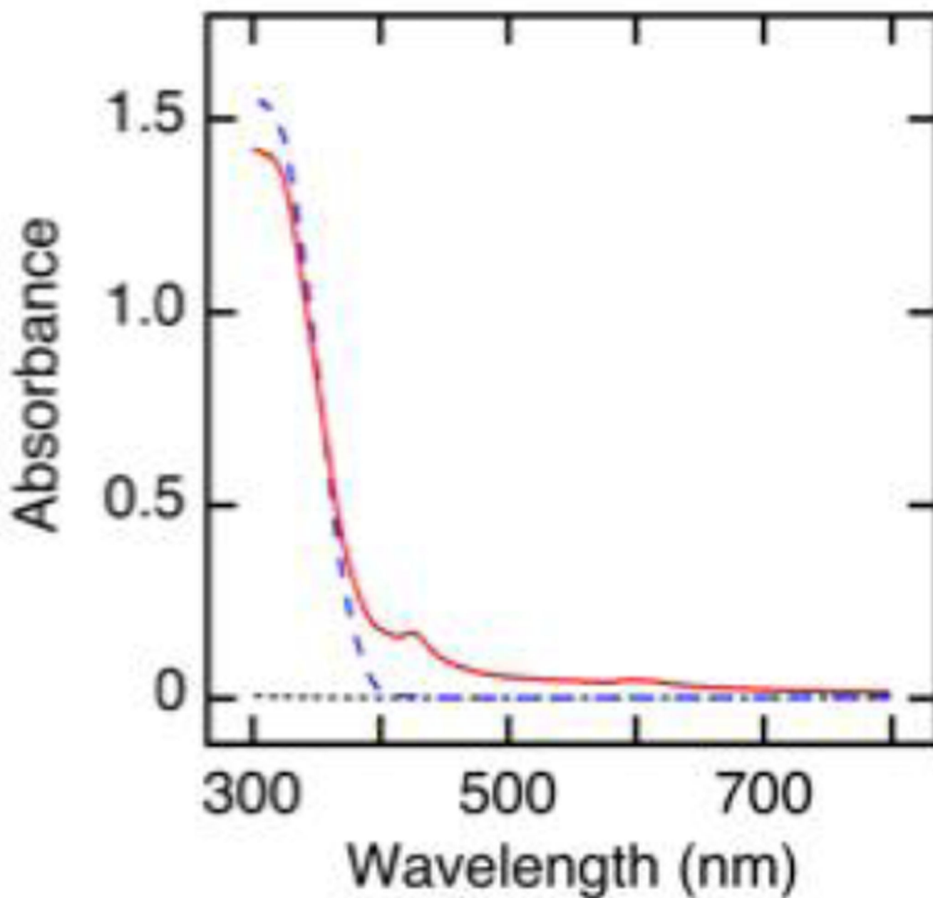
Figure 2. Absorbance spectra of \text{H}_2\text{O}_2 -etched \text{TiO}_2 nanoparticles embedded in a PDMS polymer matrix before (blue, long dashed line) and after 1-Al functionalization (red, solid line), as well as the absorption spectrum of PDMS on quartz (black, short dashed line). The absorption spectra were measured in transreflectance mode where both transmitted and reflected lights were collected employing an integrating sphere.
