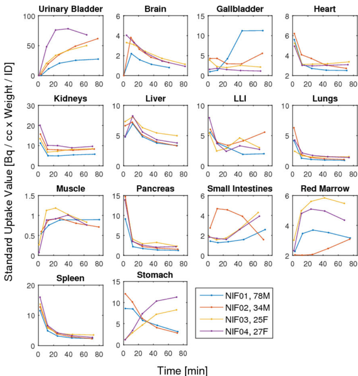
Figure 1. Source Organ Time-Activity Curves of [^{18}\text{F}] nifene in Humans
