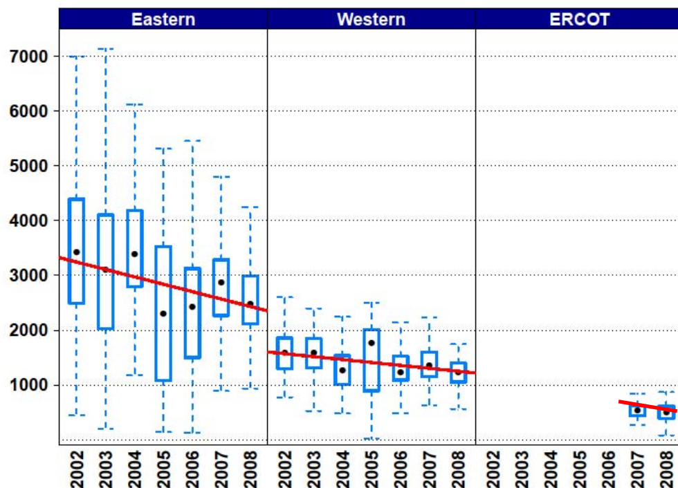
Figure ES- 1. Yearly Trends in the Frequency Response of the Eastern, Western and ERCOT Interconnections
