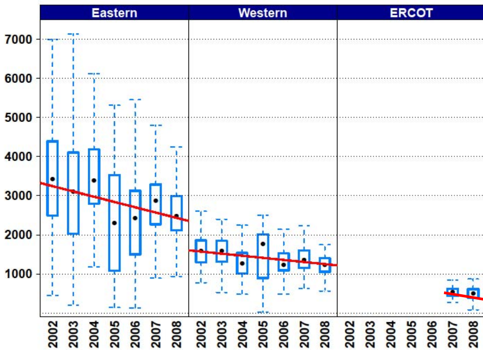
Figure 2. Yearly Trends in the Frequency Response of the Eastern, Western and ERCOT Interconnections
