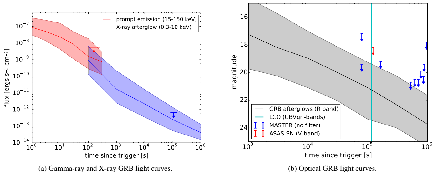
Fig. 10: The shaded bands show the gamma-ray and X-ray light curves of detected GRBs (left) and optical afterglow light curves (right). The central line shows the median flux at the indicated time and the shaded bands include 80% of all GRBs (i.e., the 10% brightest and faintest afterglows are above or below the band, respectively). The arrows show the flux upper limits from the X-ray and optical follow-up observations (see Sects. 4.1 and 4.2 for details).
