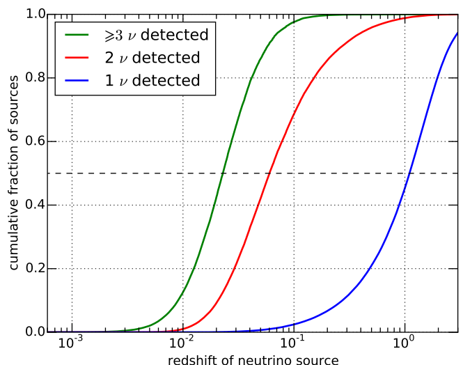
Fig. 8: Probability of detecting a neutrino source within a certain redshift. The figure was generated by simulating a population of transient neutrino sources with a density of 10^{-6} \text{Mpc}^{-3} \text{yr}^{-1} distributed in redshift according to the star-formation rate and normalized to produce the detected astrophysical neutrino flux. Sources detected with only one single neutrino are on average far away (median redshift of 1.1), while sources detected with three or more neutrinos must be located nearby.
