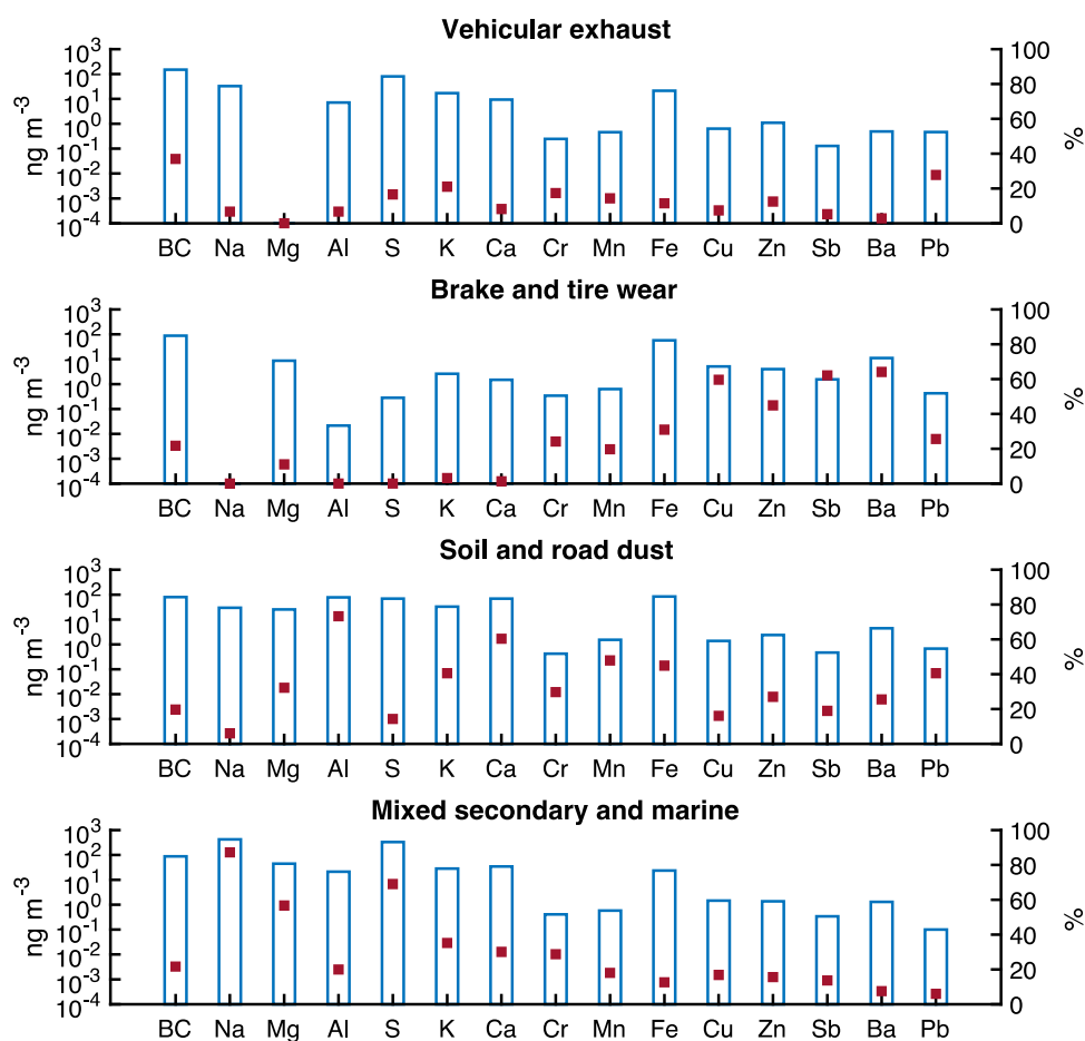
Figure 2. Factor profiles of the OP_v^{OH} PMF model. The bars (left axis) represent the concentration of species for each factor on a log scale, and the dots (right axis) denote the percentage contribution of each factor to the total concentration of each species.
