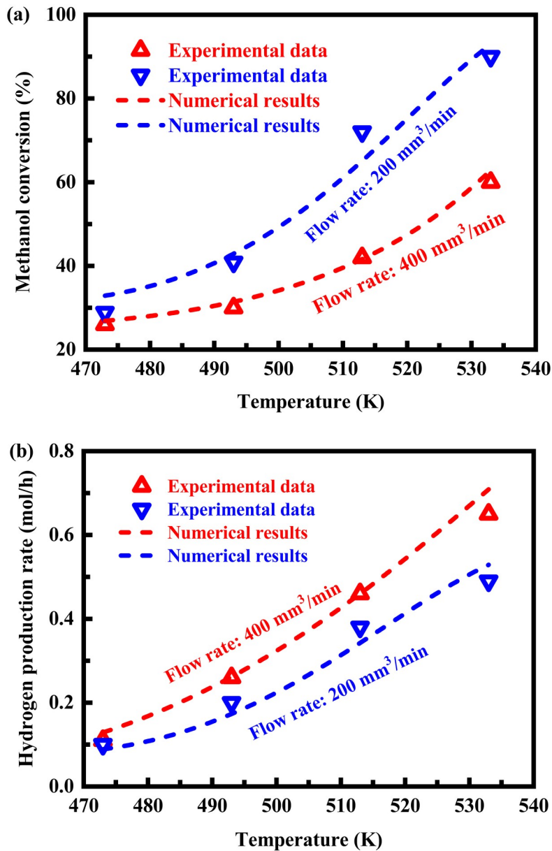
Figure 2. (a) Methanol conversion and (b) hydrogen production rate at different reaction temperatures. The experimental data [51, 52] are included for comparison.
