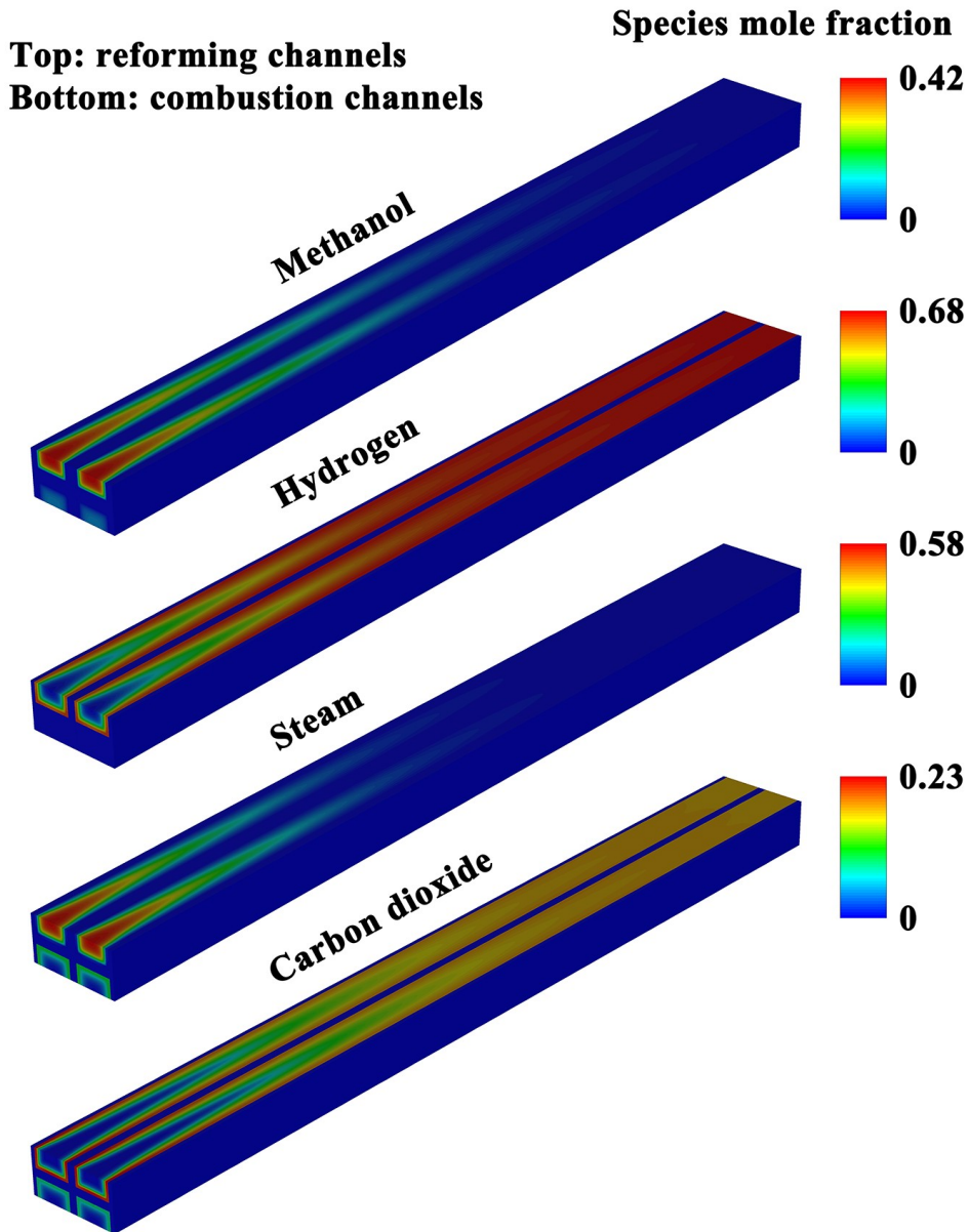
Figure 4. Contour plots of species mole fractions for the reactor. At room temperature, the thermal conductivity of the channel walls is 200 \text{ W}/(\text{m}\cdot\text{K}) .
