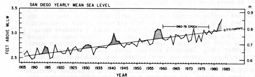
Figure 2. Secular increase in relative sea level at San Diego is close to global "average" of around 0.5 foot/century. Large positive departures are associated with major El Nino events.
