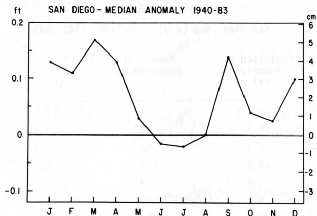
Figure 8. Median adjusted anomaly statistics, San Diego 1940-1983. Peak in September is associated with extra-tropical low pressure systems.
