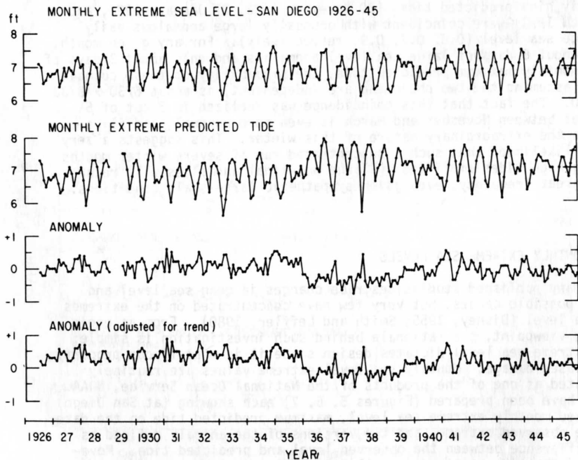
Figure 5. Monthly extreme sea level at San Diego 1926-1945 showing predicted tide on day of observed monthly maximum. Anomaly is difference between observed and predicted. Lower trace is anomaly adjusted for secular trend shown in Figure 2.
