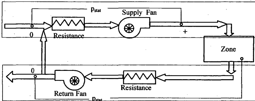
Figure 2. Diagram of VAV fan system showing sections covered by the model.
