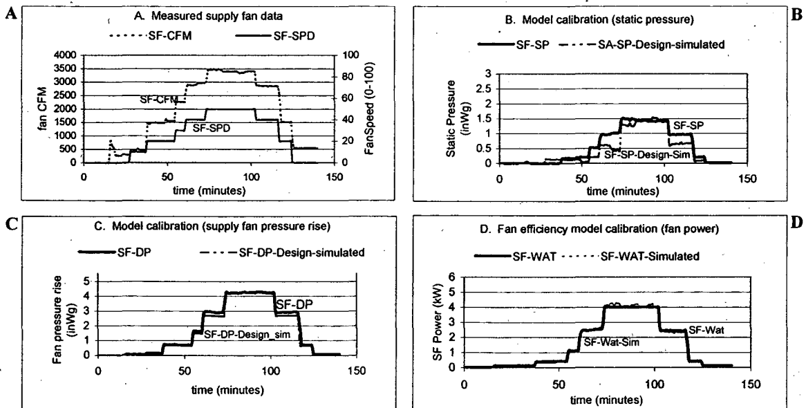
Figure 5. Supply fan calibration (experimental data).
