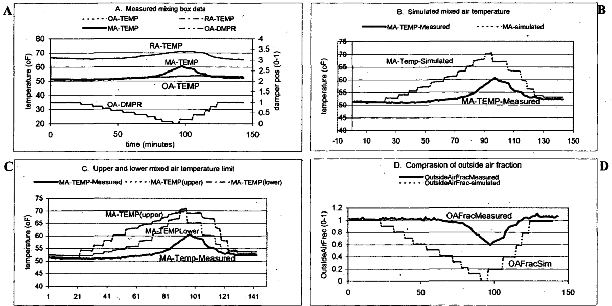
Figure 4. Mixing box fault detection (experimental data).
