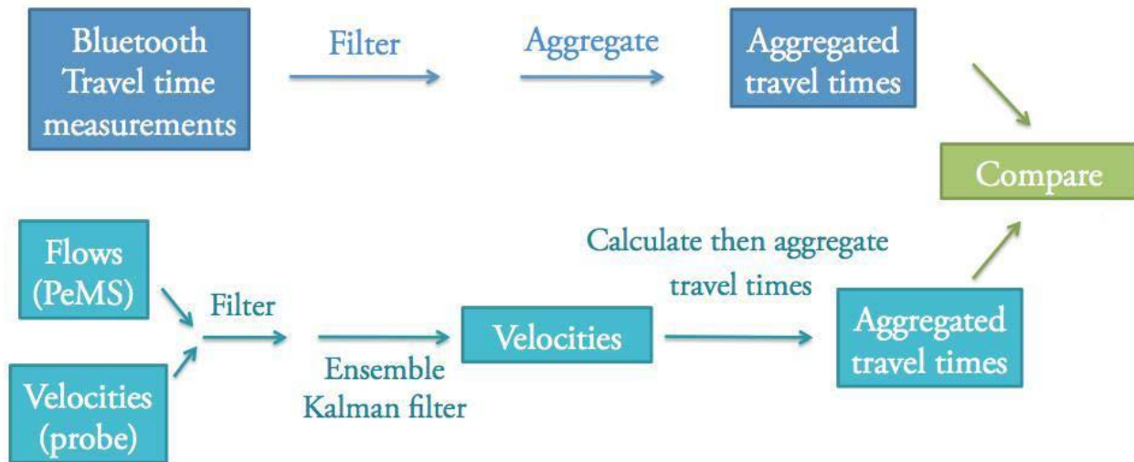
Figure 5-1: Diagram of the data flow process
