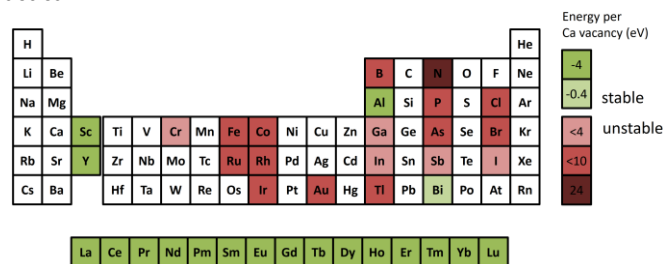
Fig. 4: Energy per Ca vacancy for the structure Ca 13 M 2 B 192 H 192 where each candidate dopant ion, M, is shown in green (stable dopant) or red (unstable dopant). Doping CaB 12 H 12 with Al, Bi, and rare-earth elements is energetically favorable.
