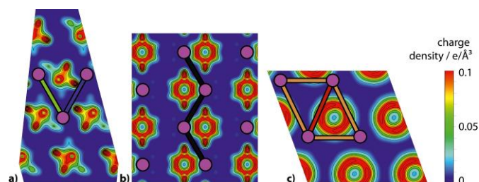
Fig. 3: Charge density of B 12 H 12 along all Ca migration paths. Ca positions (pink spheres) are shown in reference to CaB 12 H 12 . Paths are colored according to the legend in Fig. 1. Fig. a) shows the (-1.55|1.55|1) plane that is a distance of 0.73 Å distance from the origin; b) is the (1|1|0) plane with 7.37 Å distance from
