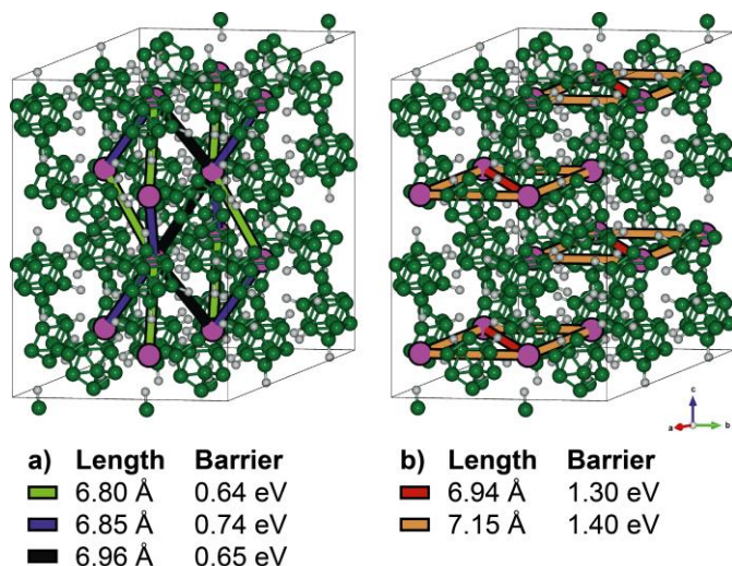
Fig. 1: \text{CaB}_{12}\text{H}_{12} structure and possible migration paths. Ca is shown as pink spheres, B as green spheres, and H as grey spheres. Possible migration paths below 9 Å are shown as lines between Ca positions. (a) Paths between layers have lower migration barriers than (b) paths in between layers.
