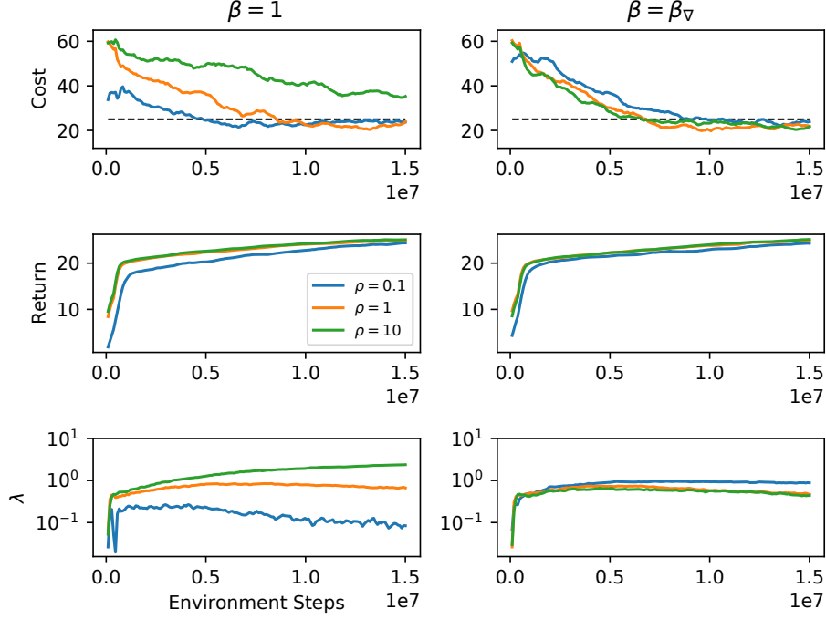
Figure 8.9: Costs, returns, and Lagrange multiplier with rewards scaled by \rho \in \{0.1, 1, 10\} ; PI-control with K_I = 1e - 3 , K_P = 0.1 . Left column : without objective-weighting, learning dynamics differ dramatically due to required scale of \lambda . Right column : with objective-weighting, learning dynamics are nearly identical. Environment: POINTGOAL1, cost limit 25.
