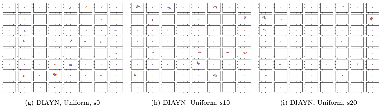
Figure 4.18: Learned behaviors in the Ant environment with uniform context distributions. Each sub-plot shows X-Y traces for five trajectories conditioned on the same context (because the learned behaviors are highly repeatable, most traces almost entirely overlap). All traces for an algorithm come from a single policy which was trained with K = 64 contexts.
