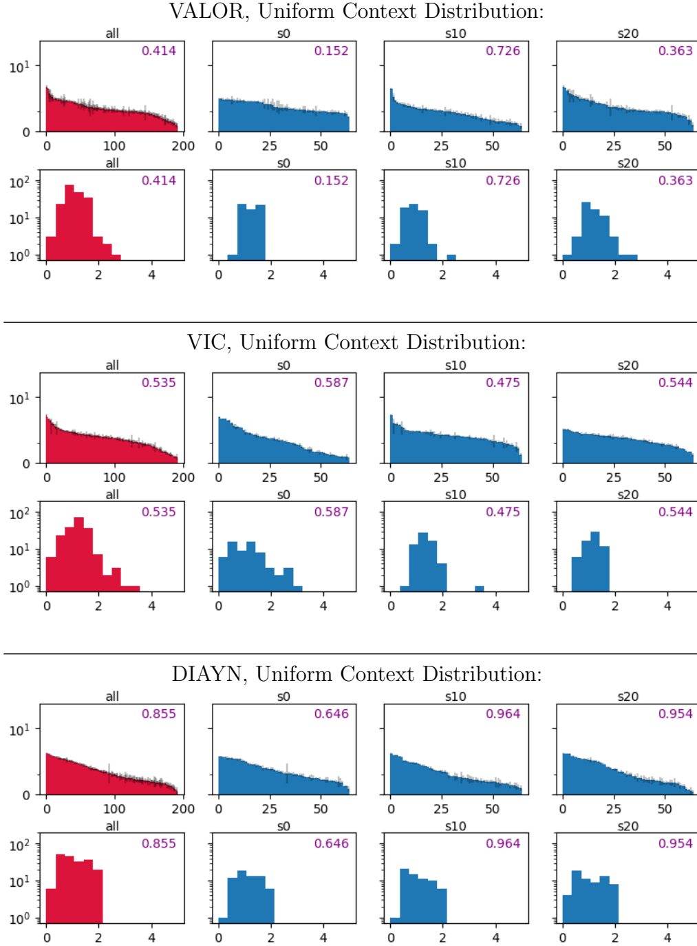
Figure 4.10: Final distance from origin in the Swimmer environment.
