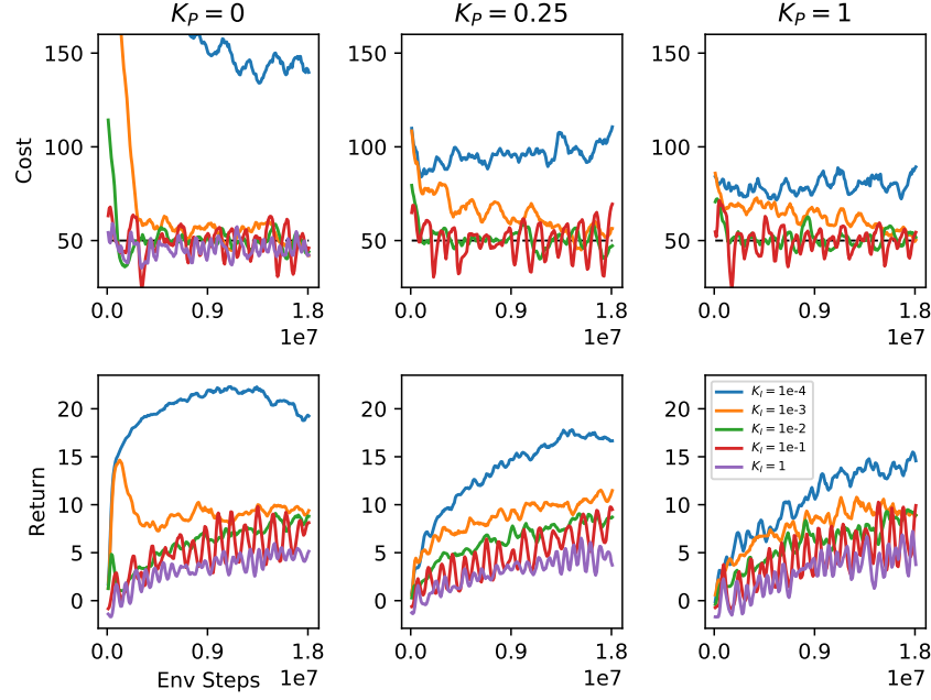
Figure 8.11: Costs and returns with varying Lagrange multiplier learning rate, K_I , and proportional control coefficient, K_P , in CARBUTTON1, cost-limit=50.
