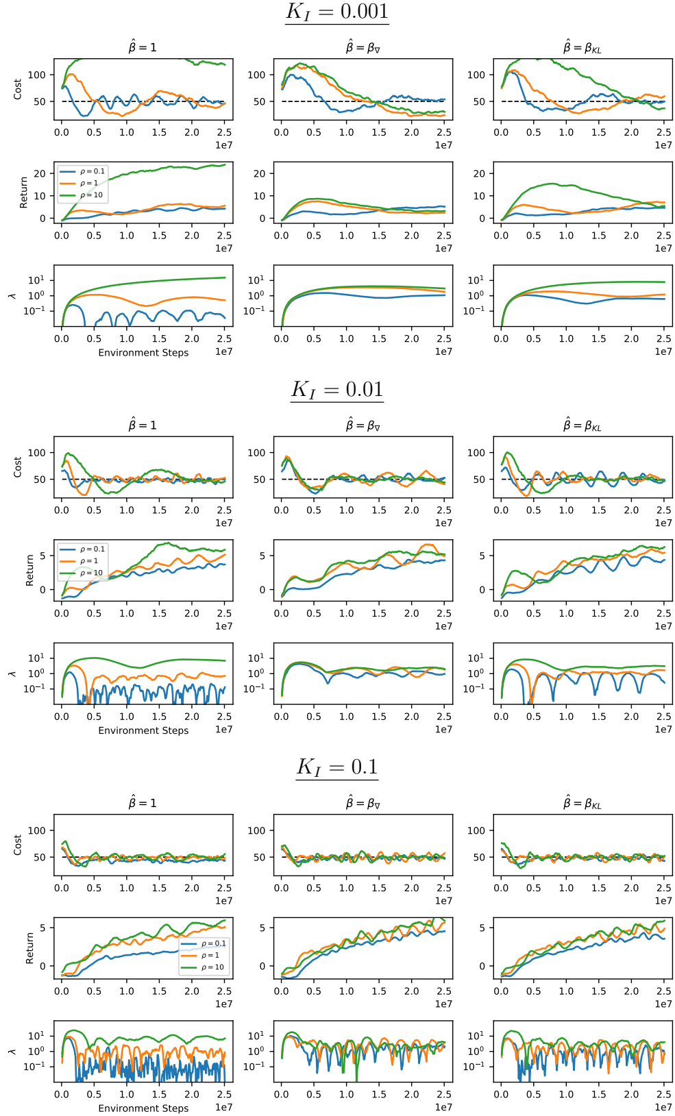
Figure 8.18: Reward scaling, I-control, DOGGOAL2, cost-limit=50.
