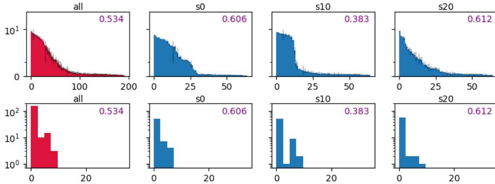
Figure 4.12: Final distance from origin in the Ant environment.
