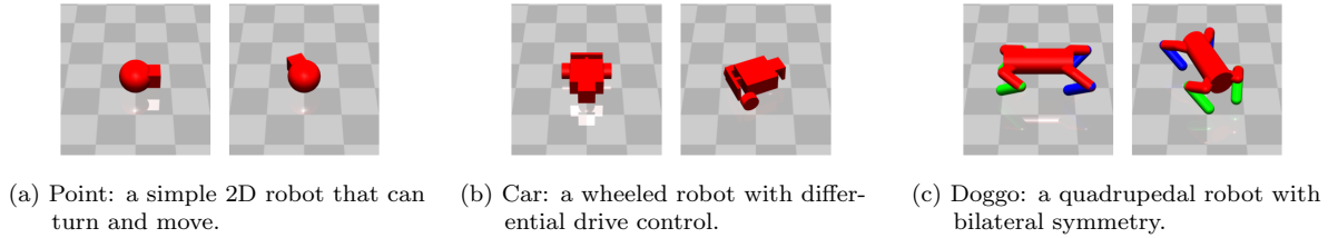
Figure 7.1: Pre-made robots in Safety Gym. These robots are used in our benchmark environments.
