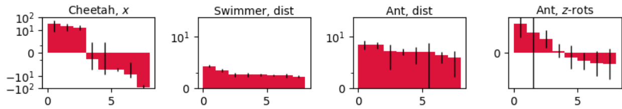
Figure 4.24: Score distributions for RR2.
