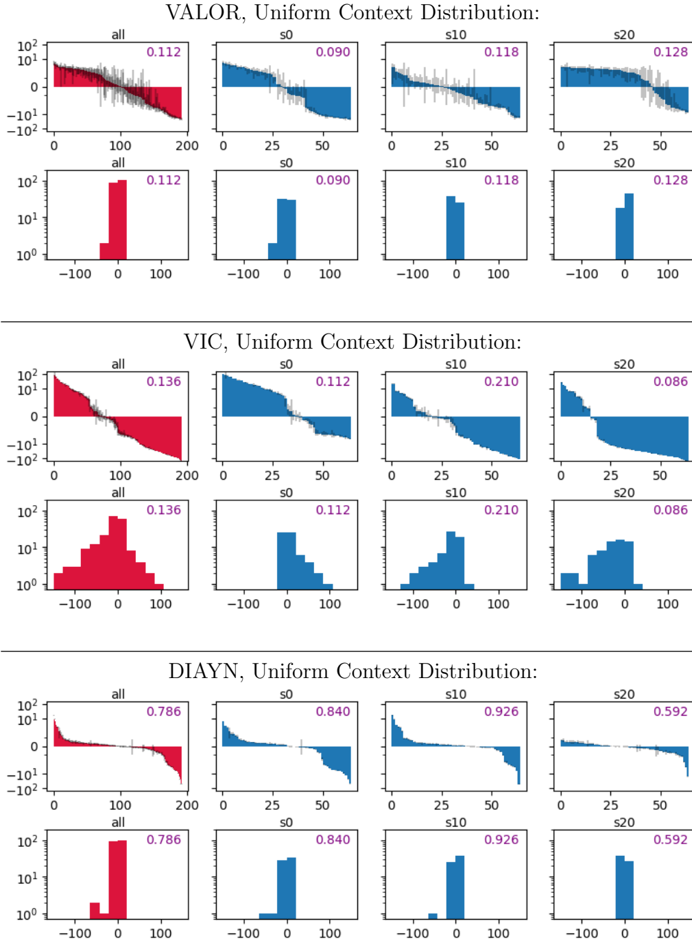
Figure 4.8: Final x -coordinate in the Cheetah environment.
