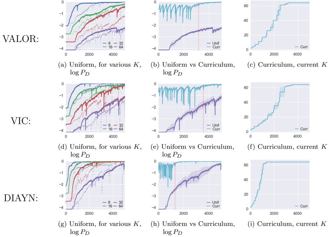
Figure 4.6: Analysis for understanding best training practices for various algorithms with HalfCheetah as the environment. The x -axis is number of training iterations, and in (a) and (b), the y -axis is E[\log P_D(c|\tau)] ; in (c), the y -axis gives the current value of K in the curriculum. (a) shows a direct comparison between learning curves with (dark) and without (dotted) context embeddings, for K \in \{8, 16, 32, 64\} . (b) shows learning performance for the curriculum approach with K_{max} = 64 , compared against the uniform distribution approach with K = 64 : the spikes and dips for the curriculum curve are characteristic of points when K changes according to Eq. 4.5. The dashed red line shows when K = K_{max} for the curriculum approach; prior to it, the curves for Uniform and Curriculum are not directly comparable, but after it, they are. (c) shows K for the curriculum approach throughout the runs from (b). All curves are averaged over three random seeds.
