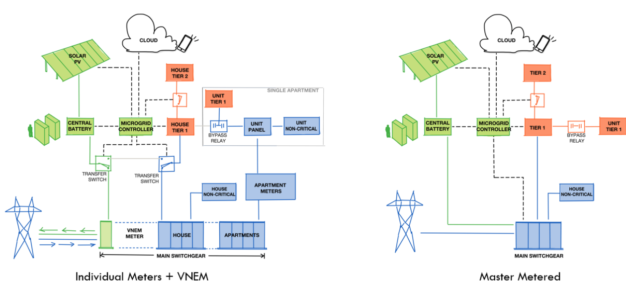
Figure 8: Left: Individual apartment electricity meter schematic with virtual net metering, and in-apartment backup power (currently allowable in CA); Right: Master metered electrical schematic to provide daily peak window power to apartments and in-apartment backup power (currently this configuration is not allowable in CA)
