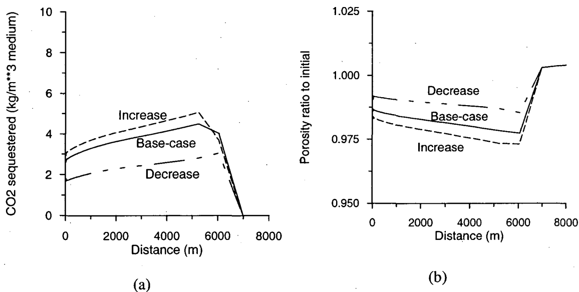
Figure 10. Cumulative \text{CO}_2 sequestered by carbonate mineral precipitation (a) and porosity ratio to initial time (b) after 10,000 years for different oligoclase kinetic rate constants.
