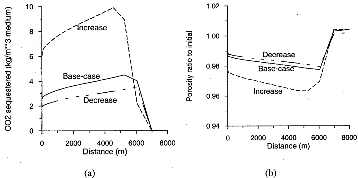
Figure 12. Cumulative CO 2 sequestered by carbonate mineral precipitation (a) and porosity ratio to initial time (b) after 10,000 years for different clinochlore kinetic rate constants.
