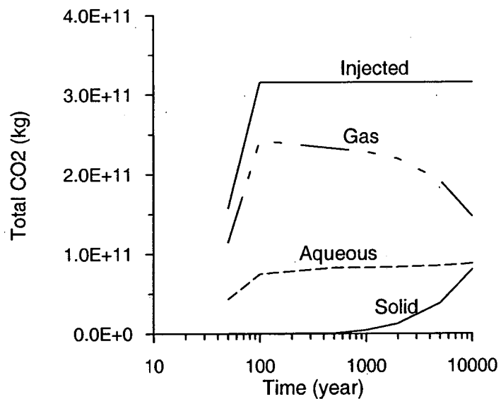
Figure 5. Total CO 2 sequestered in the three phases for the entire reservoir.
