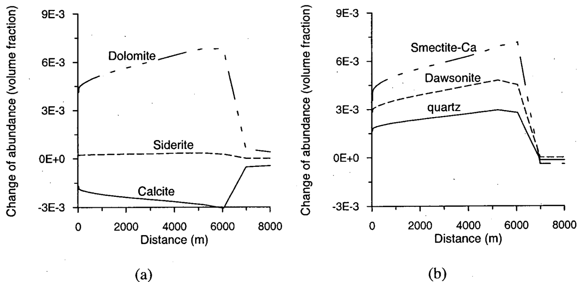
Figure 13. Change of mineral abundance after 10,000 years obtained by an increase of one order of magnitude of clinochlore kinetic rate constant.
