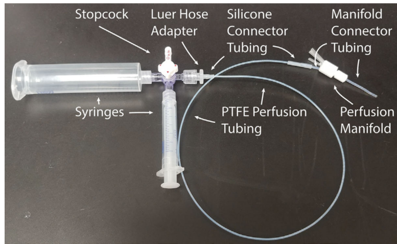
Figure 3. Homemade perfusion line.
