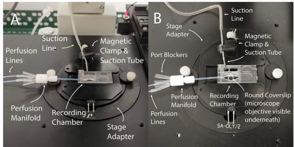
Figure 2. Assembled perfusion chamber for recording.
