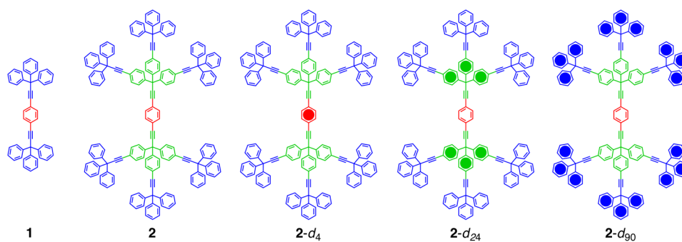
Figure 1. Structures of molecular rotor 1 , dendrimeric molecular rotor 2 , and its isotopologues 2-d 4 , 2-d 24 and 2-d 90 with the filled circles indicating perdeuterated phenylene and phenyl groups.
