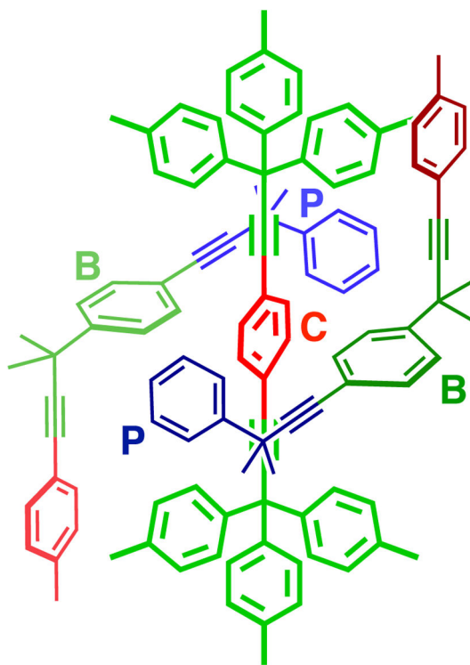
Figure 3. Schematic representation of the packing environment of the central phenylene ( C ) engaged in edge-to-face interactions acting as an acceptor with a branch phenylene ( B ) and as a donor with a peripheral ( P ) phenyl group.
