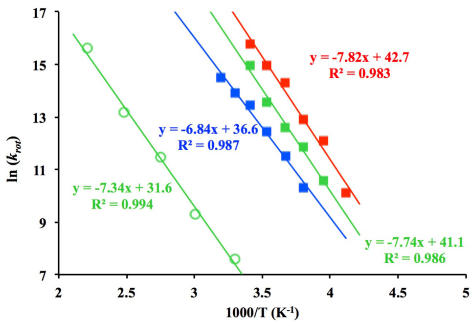
Figure 6. Arrhenius plots for crystalline (filled squares) and amorphous samples (open circles) of isotopologues of 2 .
