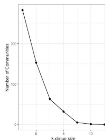
Figure 2. Number of communities uncovered via the k -clique community detection across values of k .
