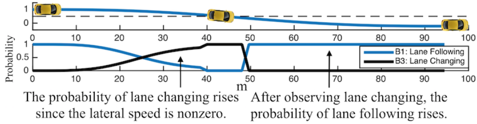
Figure 3.1: Behavior classification for a vehicle in a two-lane case.
