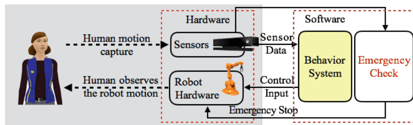
(e) Human-robot interaction platform.
