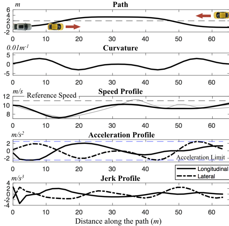
Figure 5.11: Speed profile planning for overtake.
