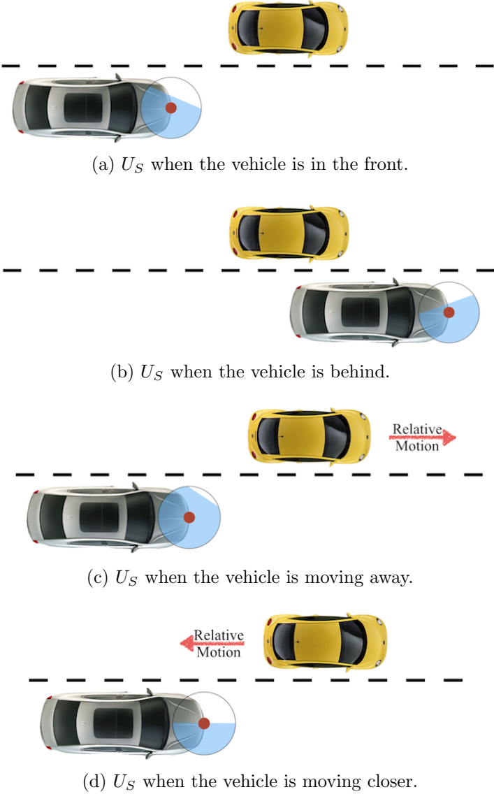
Figure 8.9: The safety constraint U_S with respect to a vehicle in the adjacent lane.
