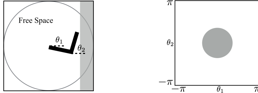
(a) The constraint in the Cartesian space. (b) The constraint in the Configuration space.
