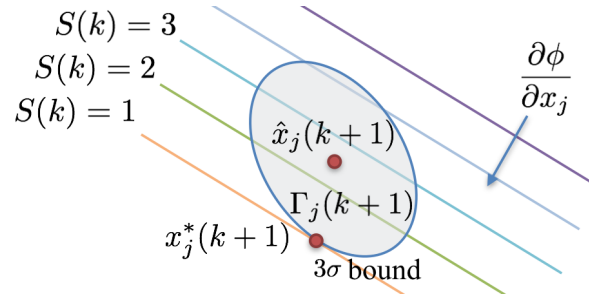
Figure 4.6: Illustration of the safety constraint in the belief space.
