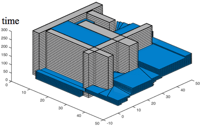
(c) The convex feasible set in time-augmented state space.
