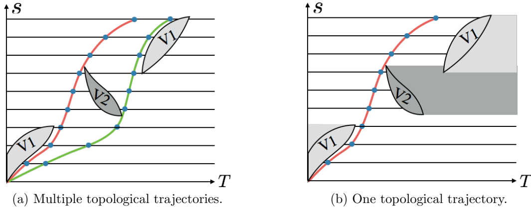
Figure 5.8: Illustration of the constraints and the topological trajectories on the s - T graph.
