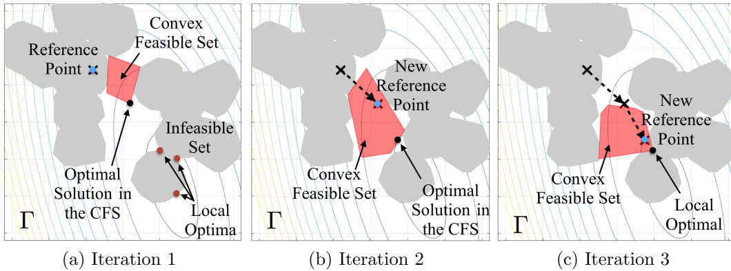
Figure 6.2: Geometry of problem 6.1 and the idea of the convex feasible set algorithm.
