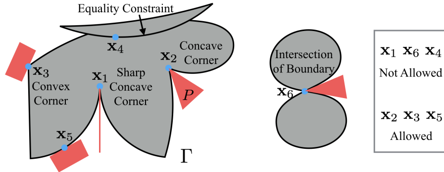
Figure 6.1: Illustration of Assumption 6.2, the geometric features of the constraint \Gamma .
