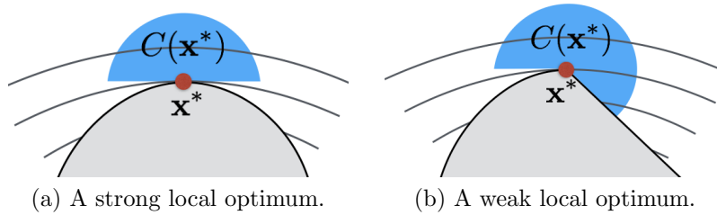
Figure 6.5: Definition of local optima.
