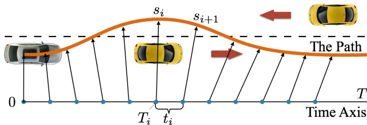
(a) Optimization over station. For each sampled time step T_i , we need to find a corresponding station s_i on the path.
