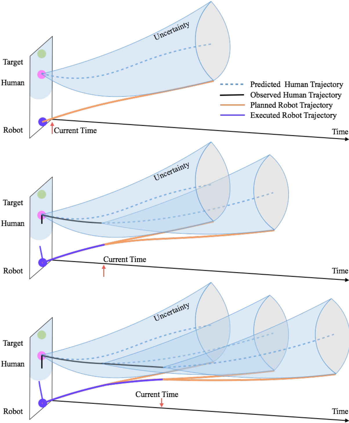
Figure 2.4: Illustration of the accumulation of uncertainty in the long term planning.
