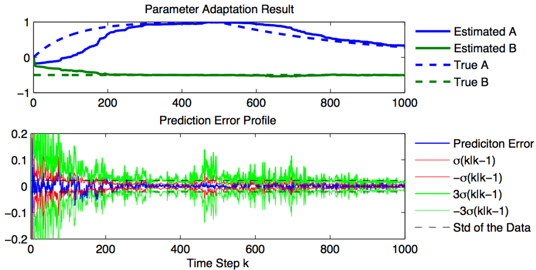
Figure 3.2: Identification of a linear time varying system.
