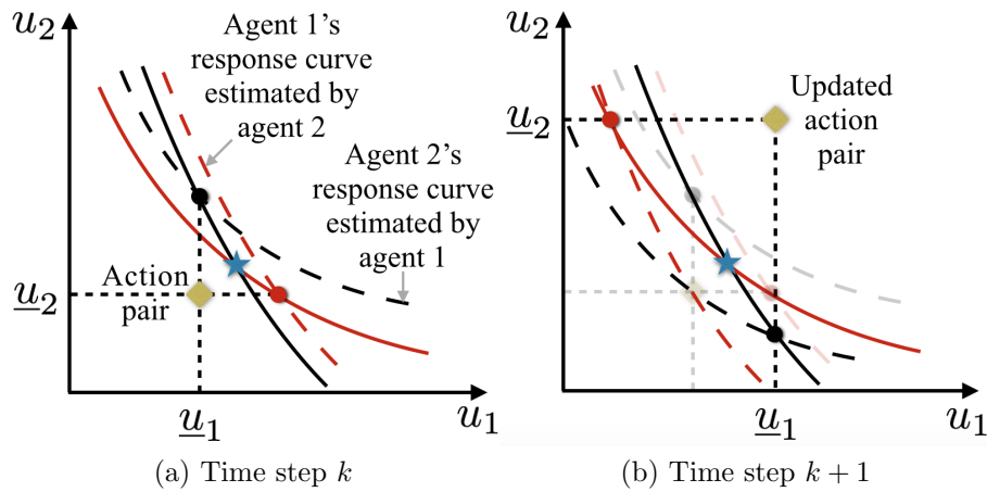
Figure 7.2: The update of the control law under the adaptive algorithm (the Blame-Me strategy)
