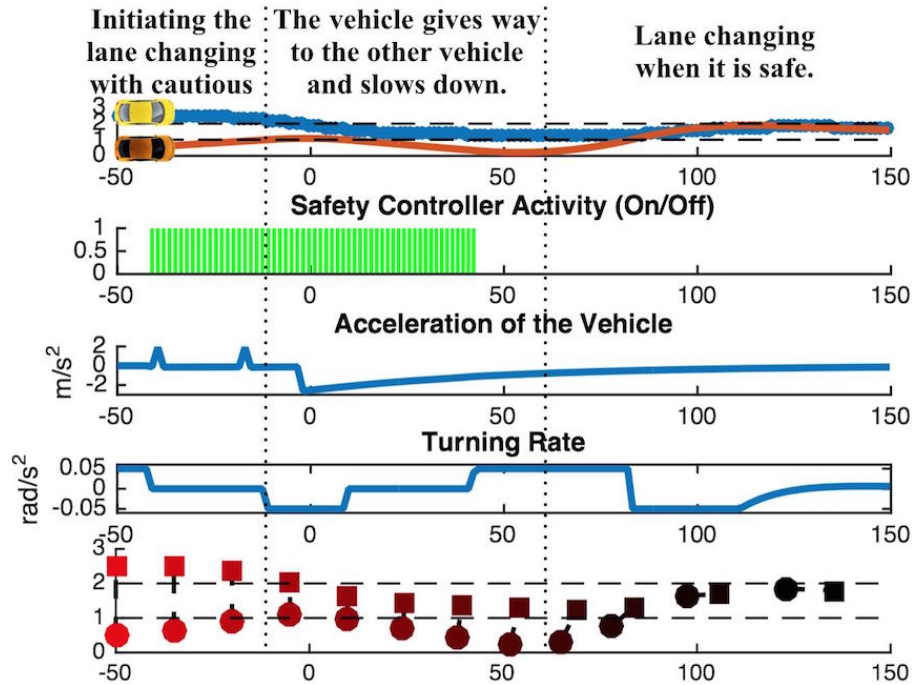
Figure 8.16: Case 3 in lane change: simultaneous lane change from opposite directions.
