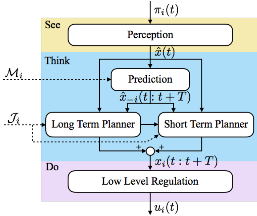
Figure 2.3: The designed architecture of the logic in this dissertation.
