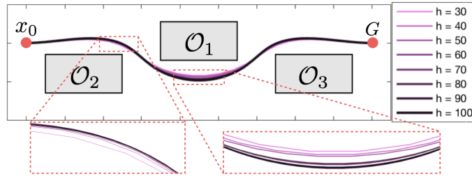
Figure 6.6: Simulation environment and the optimal trajectories for different horizon h .
