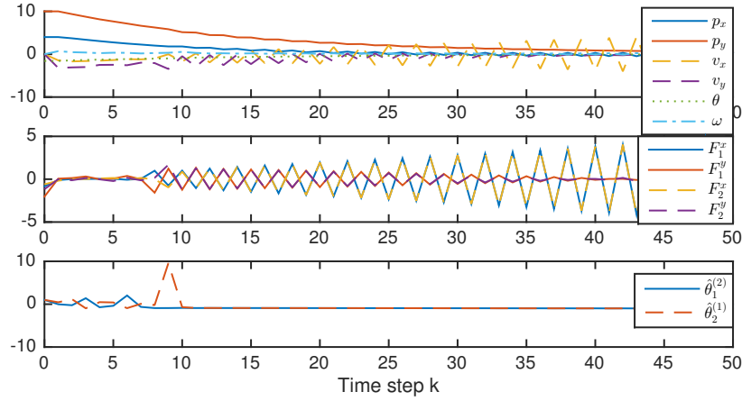
Figure 7.6: The simulation profile under the Blame-Me strategy
