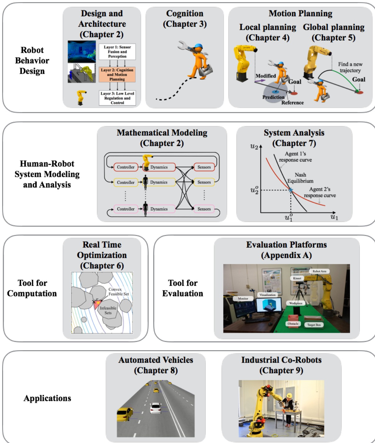
Figure 1.6: Dissertation outline.
