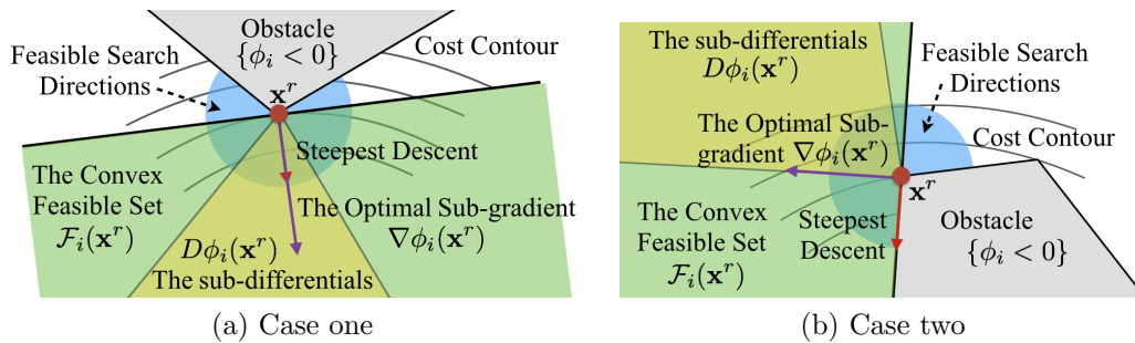
Figure 6.4: The choice of sub-gradient \hat{\nabla}\phi_i(\mathbf{x}^r) on non-smooth point \mathbf{x}^r .
