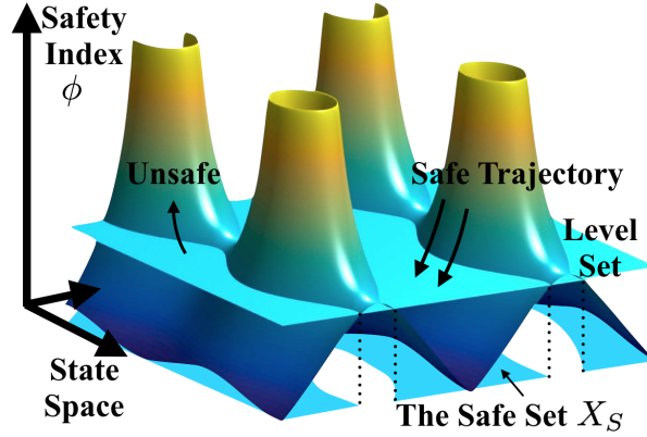
Figure 4.4: The safety index and the safe set.
