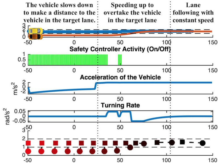
Figure 8.15: Case 2 in lane change: a slowing down vehicle in the target lane.
