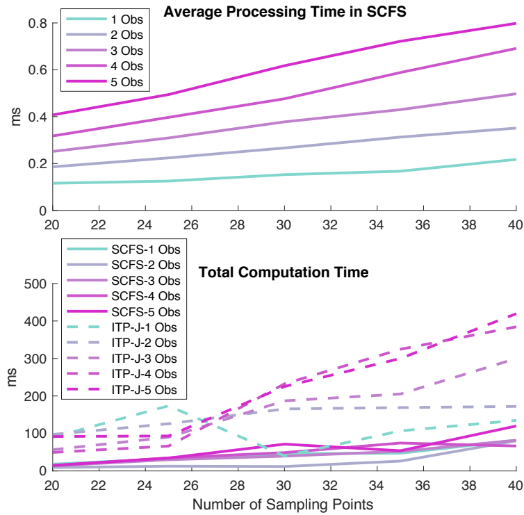
Figure 6.14: Performance of SCFS under different conditions.
