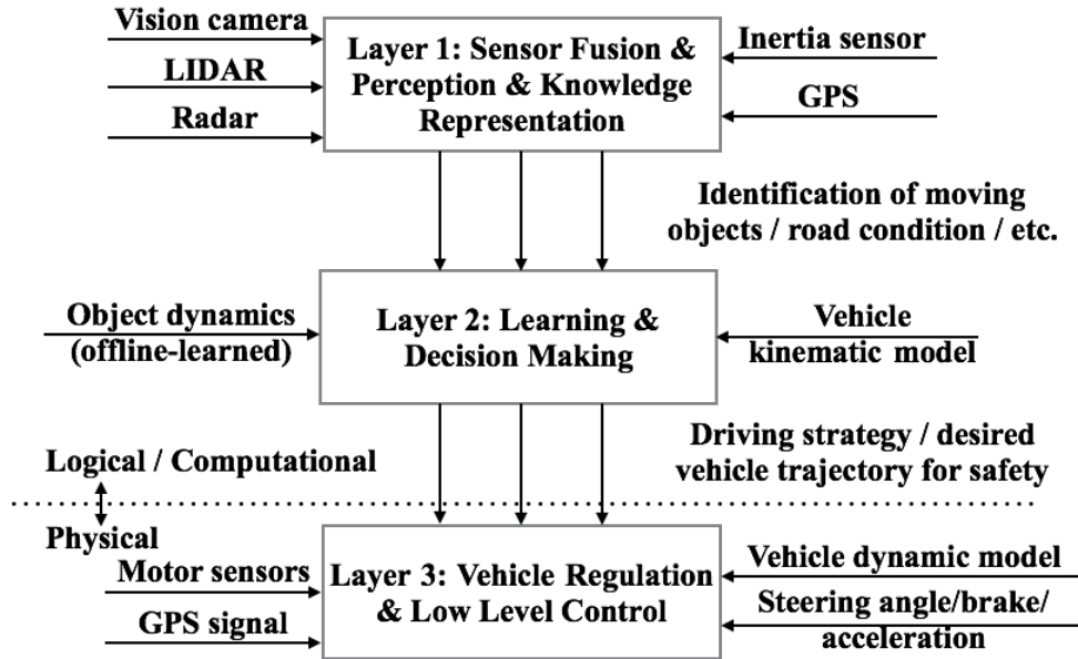
Figure 8.1: Architecture for the robustly-safe automated driving (ROAD) system
