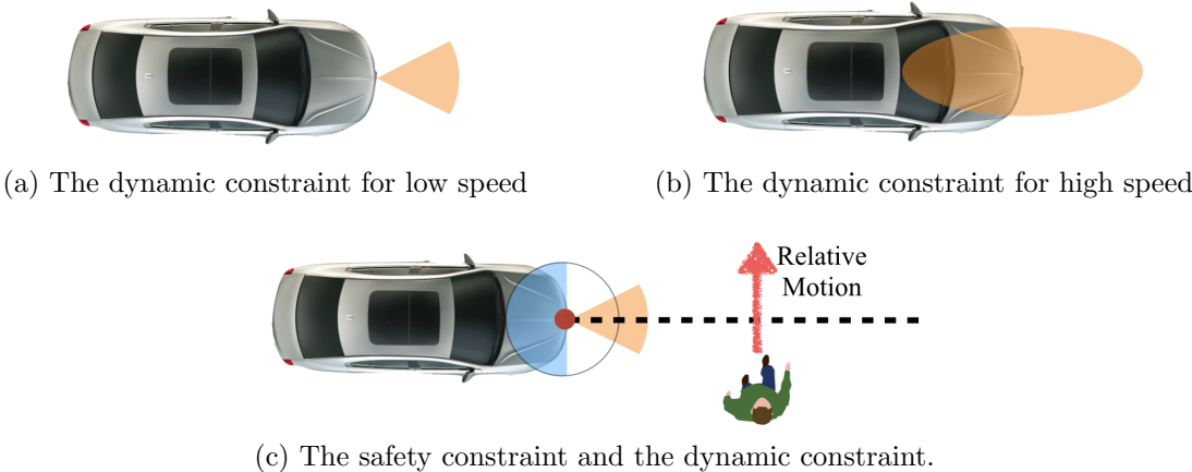
Figure 8.20: Considering the dynamic constraint together with the safety constraint.
