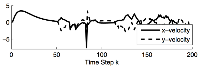
(c) The velocity profile of the robot.
