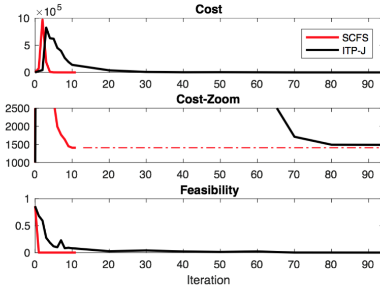
Figure 6.13: Profiles of cost and feasibility in SCFS and ITP-J.
