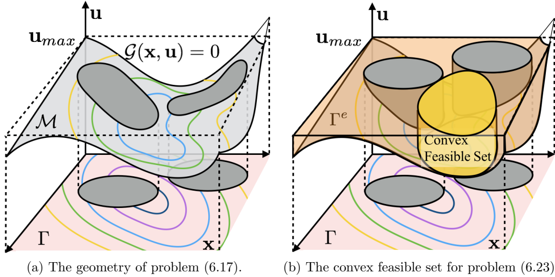
Figure 6.9: Geometric illustration of the non-convex optimization on a nonlinear space.
