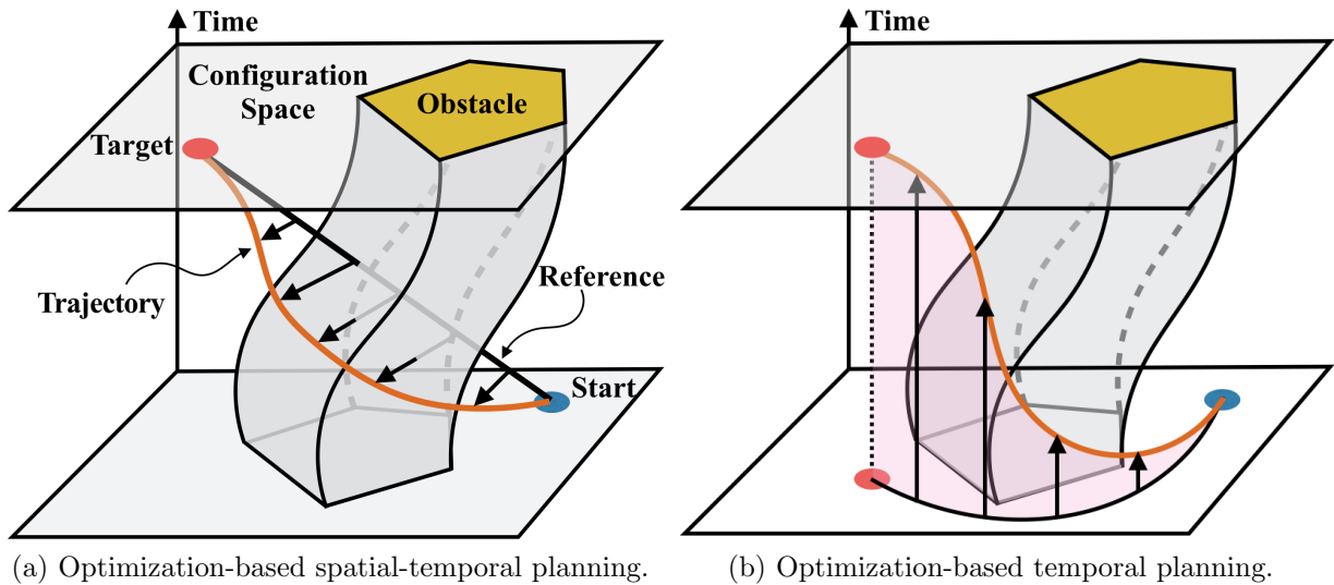
Figure 5.1: The global motion planning problem and typical methods.
