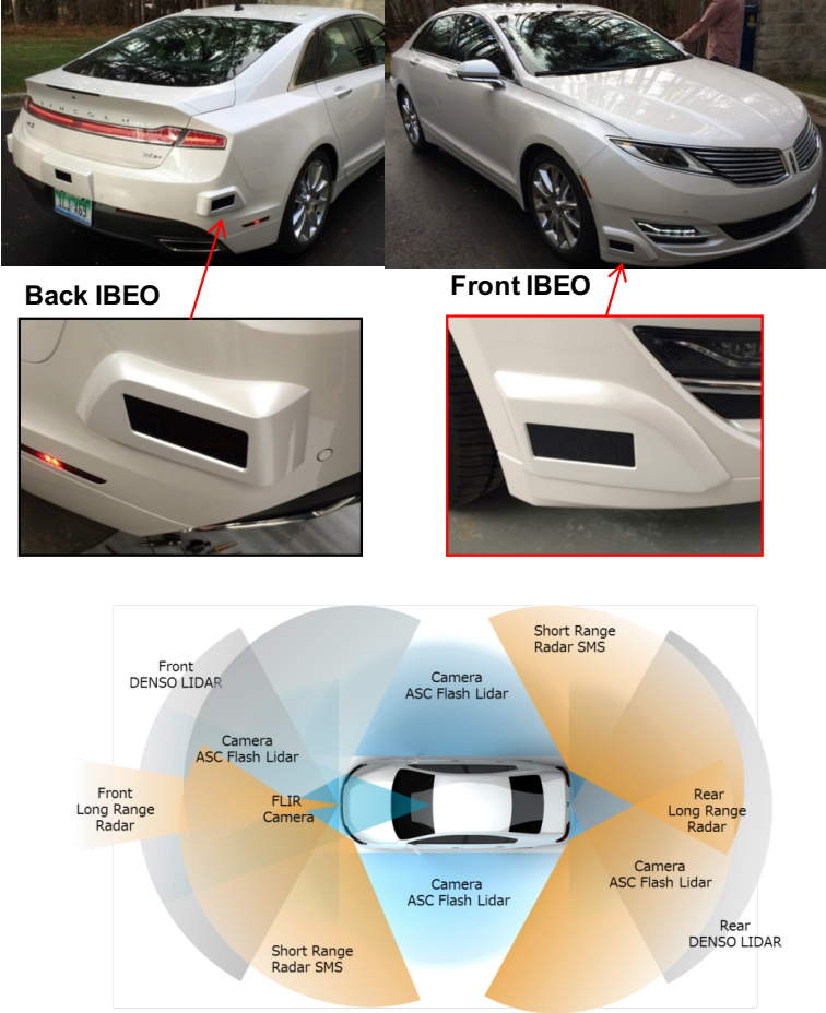
Figure 8.10: The test vehicle: Lincoln MKZ.
