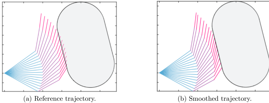
Figure 5.5: Trajectory smoothing for a robot arm.
