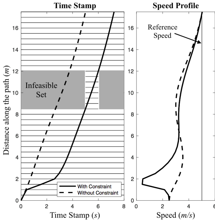
(b) Comparison between the speed profiles with and without the temporal constraint.
