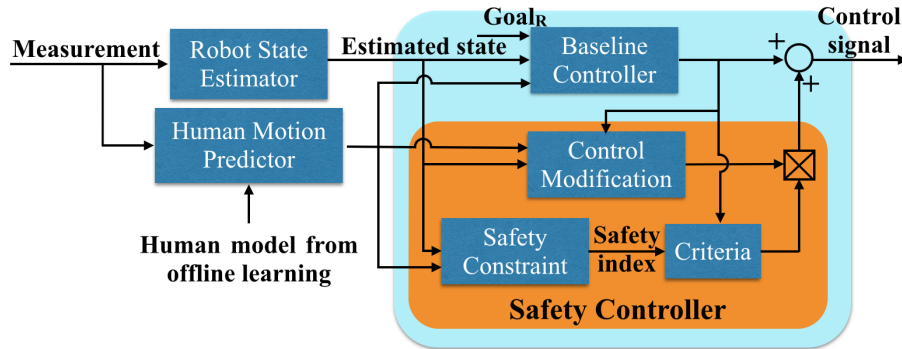
Figure 9.2: The controller architecture.
