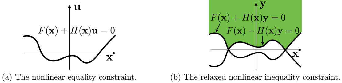
Figure 6.10: The relaxation of the nonlinear equality constraint.
