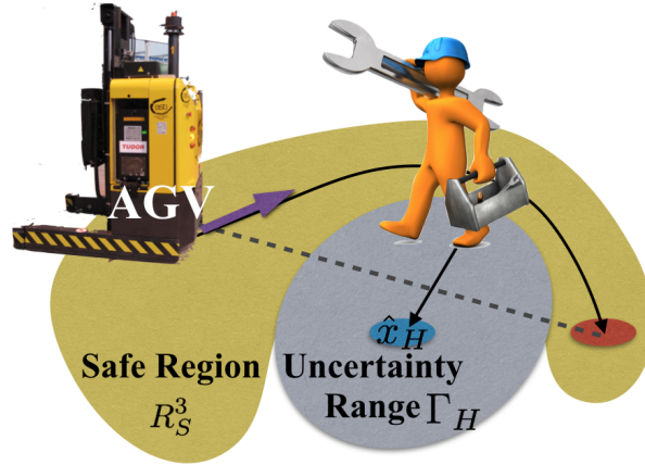
Figure 4.3: Solving the conflicts by re-planning in the safe region R_S^3 .
