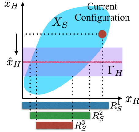
Figure 4.2: Illustration of the state space safety constraints X_S , R_S^1 , R_S^2 and R_S^3 .
