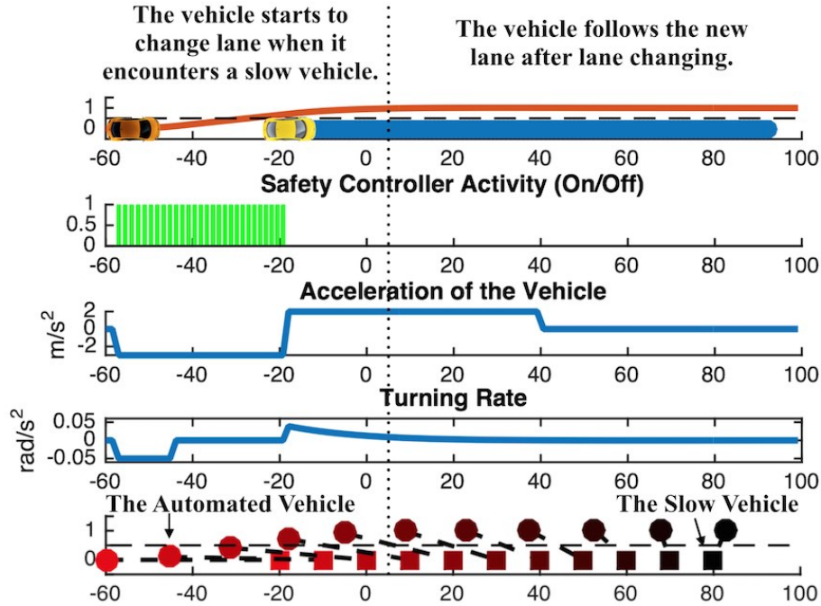
Figure 8.12: Case 2 in lane following: slow front vehicle.
