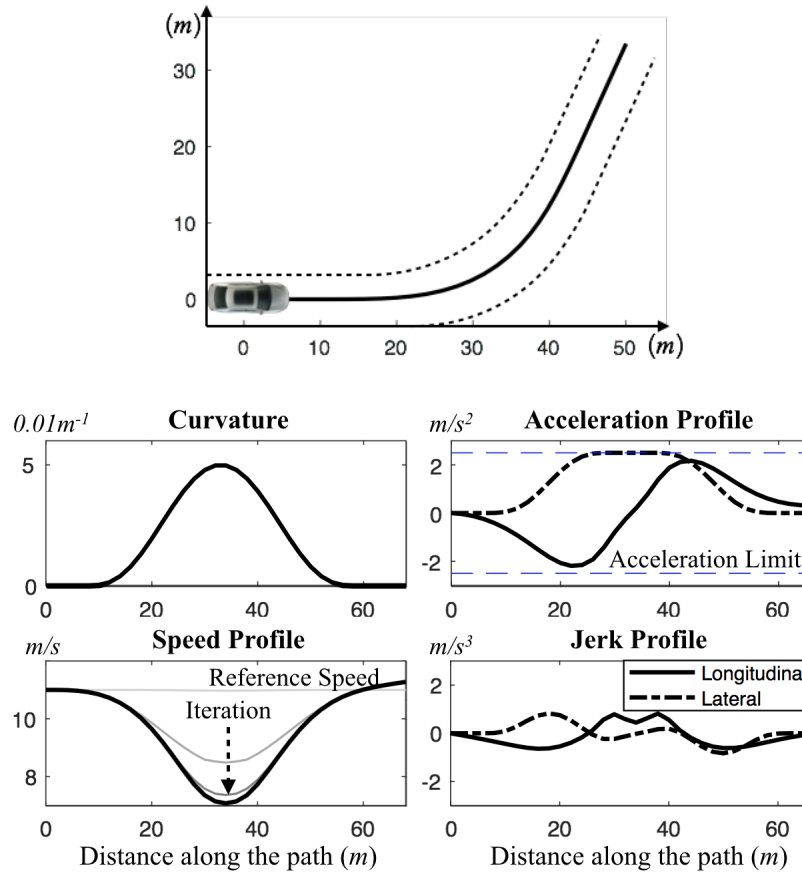
Figure 5.10: Speed profile planning for driving on a curvy road.
