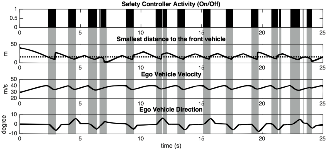
(b) The distance and velocity profile for mixed traffic simulation.
