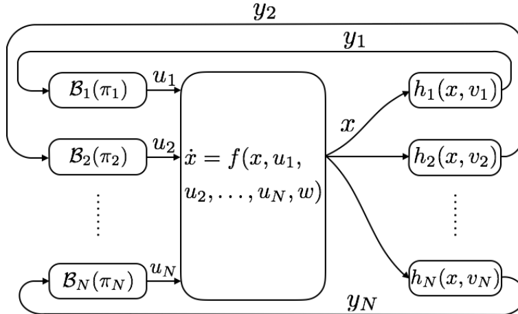
Figure 2.1: The block diagram of the multi-agent system.
