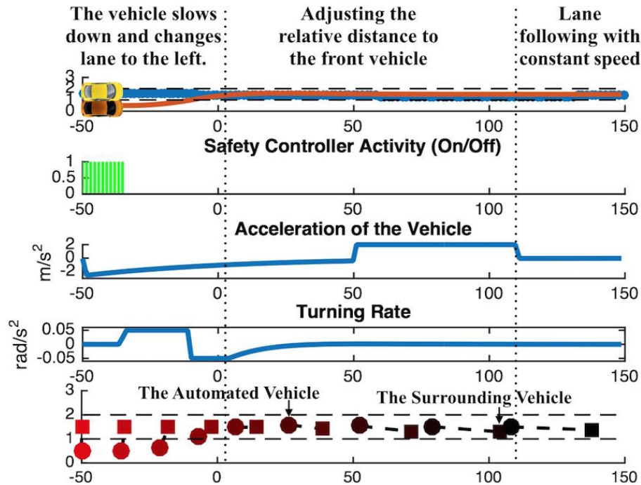
Figure 8.14: Case 1 in lane change: a parallel vehicle in the target lane.
