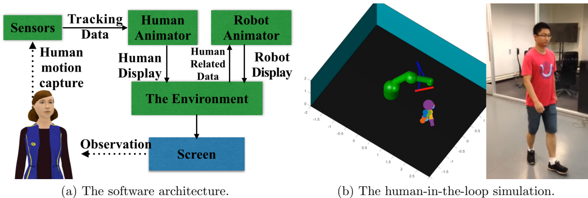
Figure A.3: The human-in-the-loop simulation platform for industrial robots.
