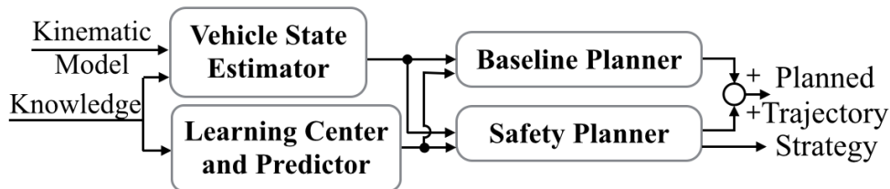
Figure 8.7: The structure of the decision making center.
