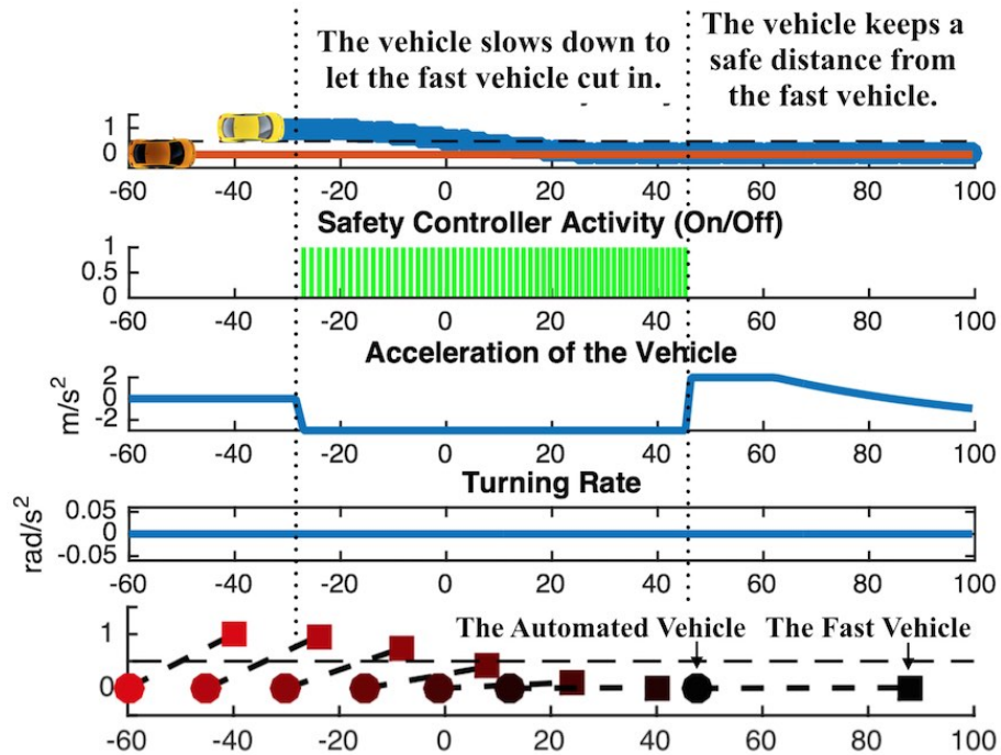
Figure 8.13: Case 3 in lane following: fast cut-in vehicle.
