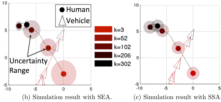
Figure 4.7: Application of the SEA algorithm and the SSA algorithms on an AGV.
