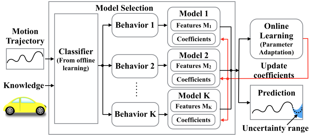
Figure 8.5: The structure of the learning and prediction center.
