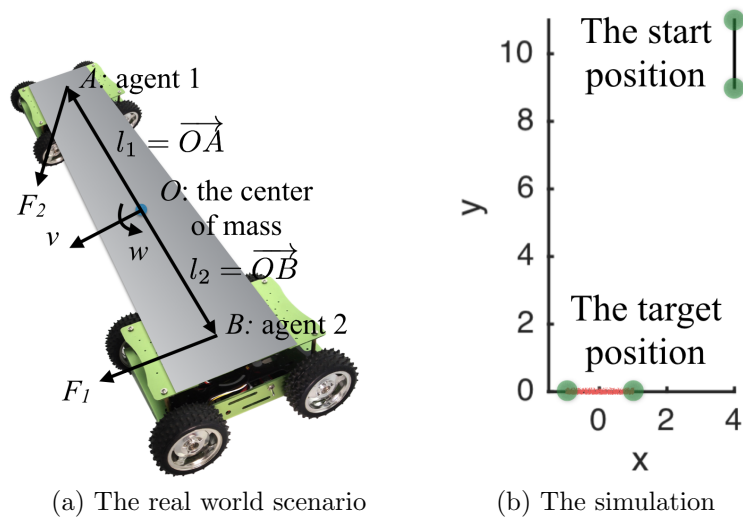
Figure 7.4: Multi-robot cooperation
