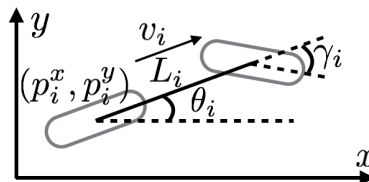
Figure 8.3: The kinematic bicycle model.
