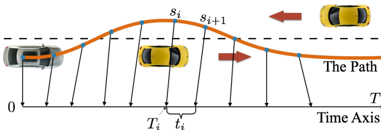
(b) Optimization over time. For each sampled station s_i , we need to find a corresponding time stamp T_i on the time axis.
