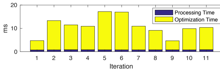
Figure 6.12: Decomposition of the computation time in SCFS.
