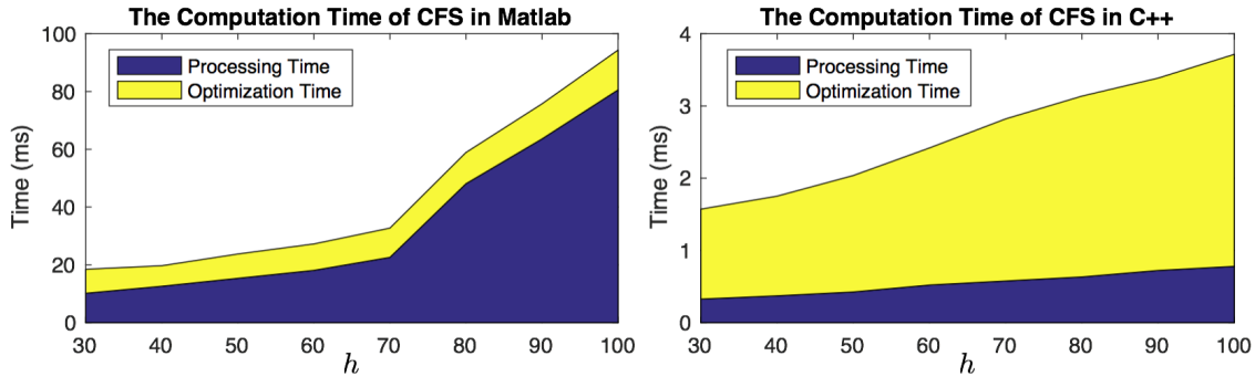
Figure 6.7: The decomposed time per iteration using Algorithm 6.1.
