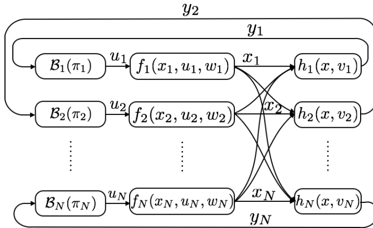
Figure 2.2: The block diagram of the decomposable multi-agent system.
