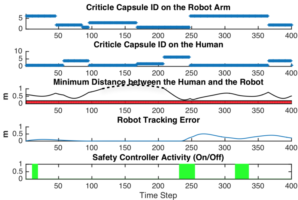
Figure 9.7: The simulation profile of the 6DoF robot arm
