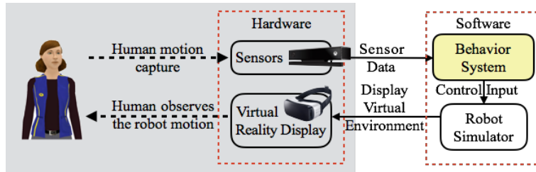
(a) Virtual reality-based human-in-the-loop platform.
