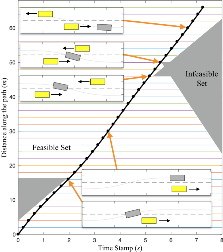
Figure 5.12: The optimal time stamps for overtake.
