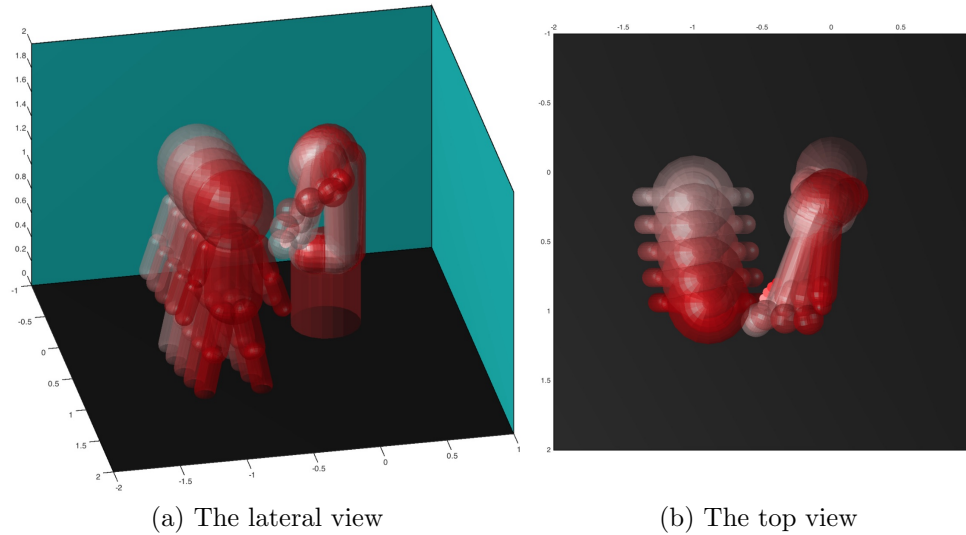
Figure 9.8: The simulated response of the 6DoF robot arm: scenario 1
