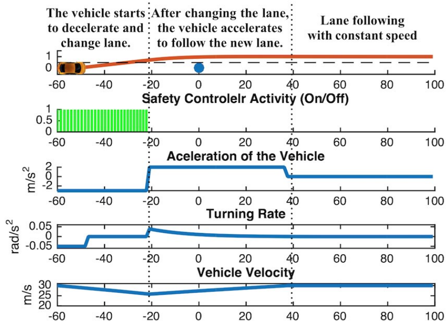
Figure 8.11: Case 1 in lane following: stationary obstacle.
