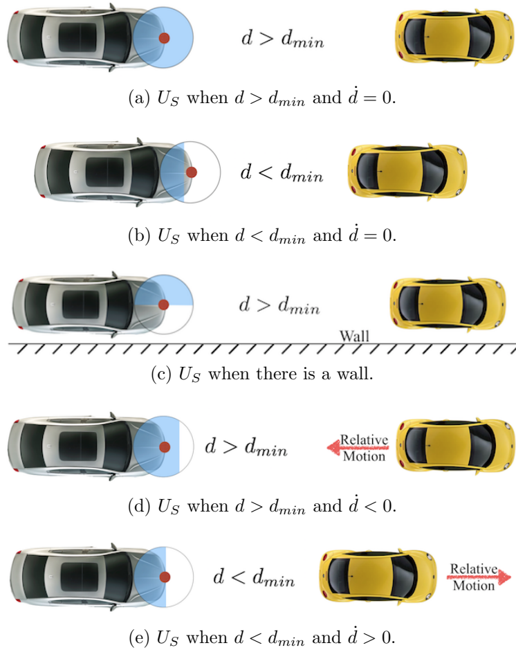
Figure 8.8: The safety constraint U_S with respect to a front vehicle.
