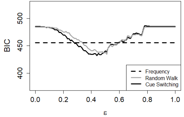
Figure 3. Performance of the models of retrieval on unweighted semantic networks at increasing thresholds \varepsilon . switching model.
