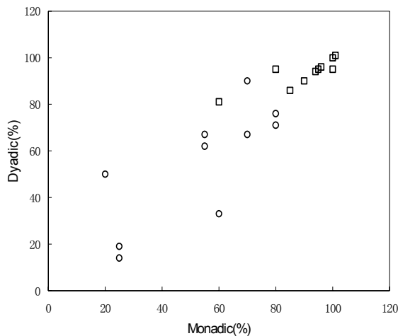
Figure 4. A scatter plot of English data.
