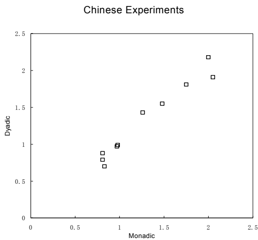
Figure 1. Cross tabulations of schema weights.
