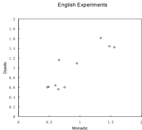
Figure 2. Cross tabulations of schema weights.
