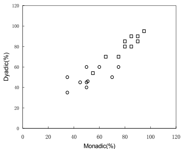
Figure 3. A scatter plot of Chinese data
