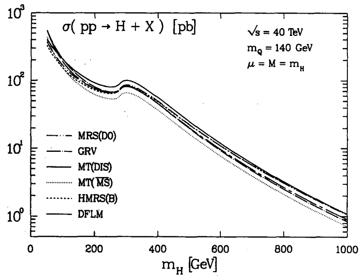
Figure 3: The spread of the Higgs production cross section for various parametrizations [14,16] of the parton densities. (a) LHC and (b) SSC for a top quark mass of 140 GeV.
