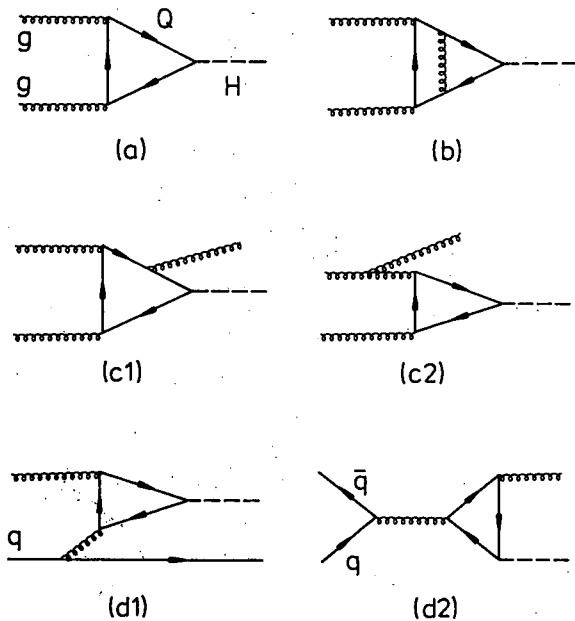
Figure 1: Generic diagrams for the production of Higgs bosons in gluon-gluon, gluon-quark and quark-antiquark collisions: (a) lowest order gg contribution; (b) vertex corrections; (c) real gluon radiation; (d) Higgs production in qg and q\bar{q} collisions.
