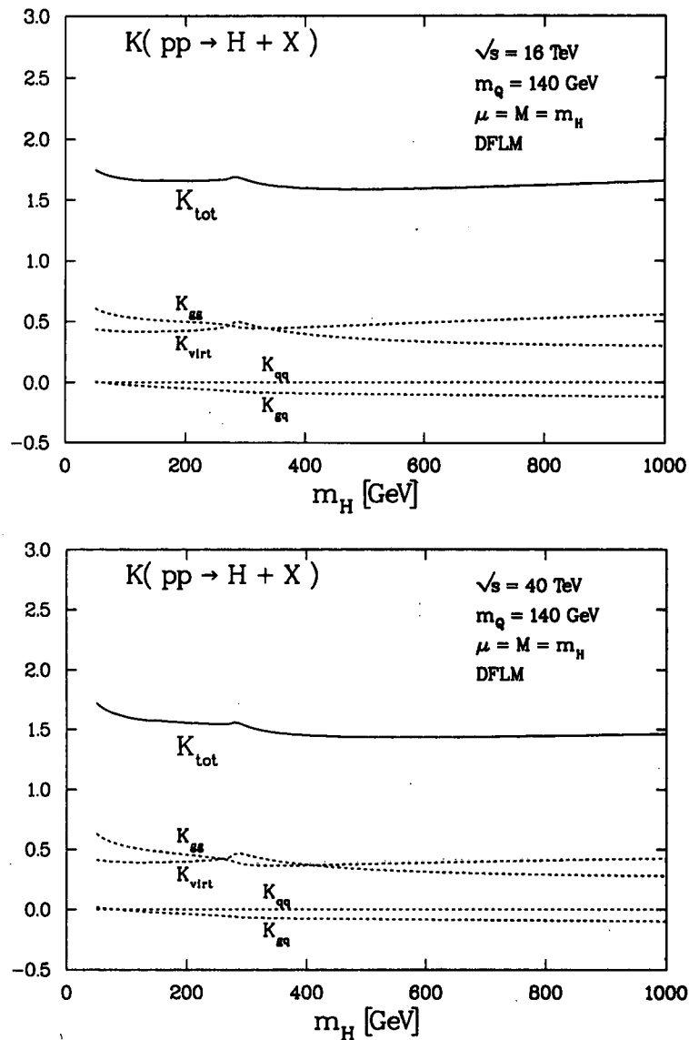
Figure 2: K factors of the QCD corrected cross sections \sigma(pp \rightarrow H) ; K_{virt} : regularized virtual corrections, K_{AB} : real corrections [ A, B = g, q ], K_{tot} : ratio of the QCD corrected cross section to the lowest order cross section. (a) LHC with \sqrt{s} = 16 TeV, (b) SSC with \sqrt{s} = 40 TeV.
