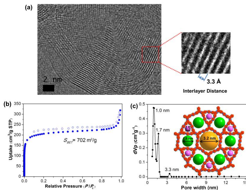
Fig. 2. (a) HRTEM image of the htb type BITA-PDA COF showing the interlayer packing structure. (b) N 2 adsorption (●) and desorption (○) isotherm curves at 77 K and (c) pore size distribution profile of BITA-PDA COF.
