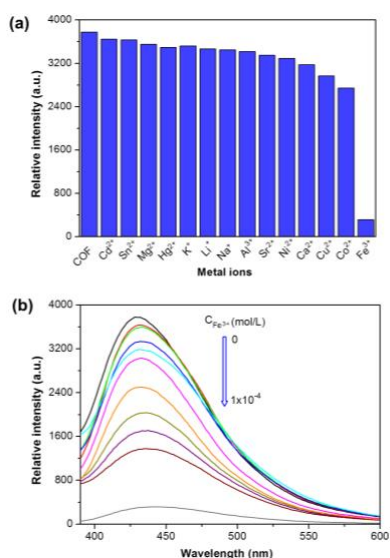
Fig. 3. (a) Comparison of fluorescence intensity of BITA-PDA COF in the presence of various metal ions ( 1 \times 10^{-4} mol/L) in DMF ( \lambda_{\text{ex}} = 322 nm). (b) Emission spectra of BITA-PDA COF in DMF suspensions containing various C_{\text{Fe}^{3+}} (0 to 1 \times 10^{-4} mol/L).
