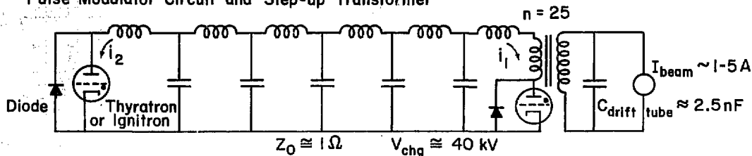
Pulse Modulator Circuit and Step-up Transformer
