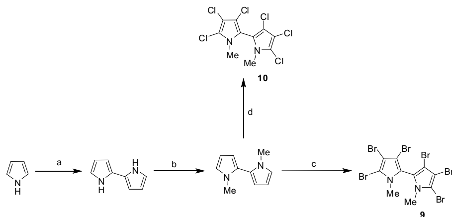
Scheme 2. Reagents and conditions: (a) pyrrole (3 equiv.), PIFA (1 equiv.), TMSBr (2 equiv.), DCM, -78^{\circ}\text{C} to -40^{\circ}\text{C} , 1h (b) \text{CH}_3\text{I} (2.2 equiv.), NaH (3.0 equiv.), DMF, 0^{\circ}\text{C} , 1h (c) NBS (7.0 equiv.), \text{CH}_3\text{CN} , -40^{\circ}\text{C} to 25^{\circ}\text{C} , 15 h. (d) NCS (6.2 equiv.), \text{CH}_3\text{CN} , -40^{\circ}\text{C} to 25^{\circ}\text{C} , 90 min.
