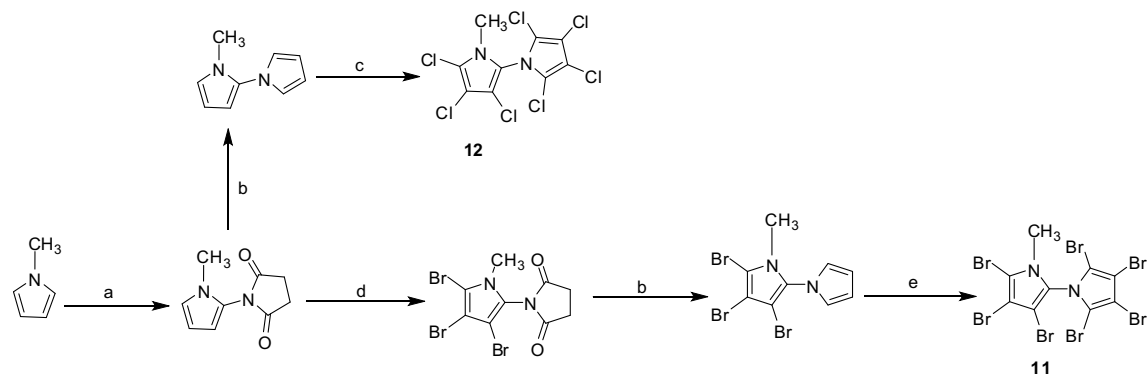
Scheme 3. Reagents and conditions: (a) NCS, \text{NaHCO}_3 , DCM, dark, rt, 4 h (b) \text{HSi}(\text{OEt})_3 , \text{Ti}(\text{O}i\text{Pr})_4 , benzene, 65^{\circ}\text{C} (c) \text{SO}_2\text{Cl}_2 , DCM, rt, 3 h (d) NBS (3.6 equiv.), THF, -78^{\circ}\text{C} to 25^{\circ}\text{C} , 3 h (e) bromine, chloroform, rt, 4 h.
