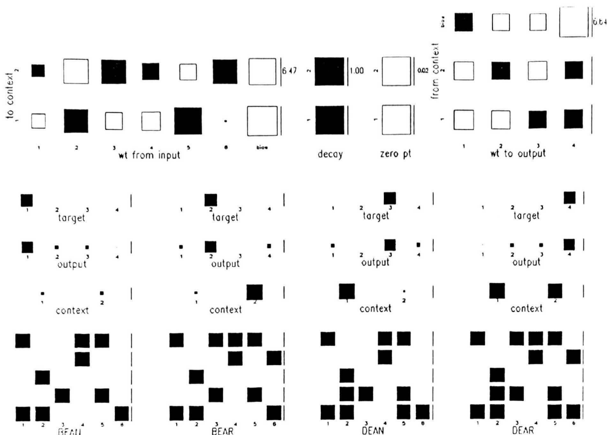
Figure 2. The DEAR/DEAN/BEAR/BEAN problem. The upper half of the figure shows learned weights in the network, the lower half activity levels in response to each of the four input sequences.
