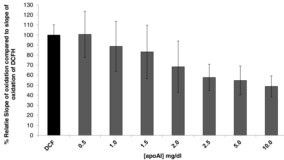
Figure 6 The effect of purified, commercially available, lipid-free apolipoprotein AI (ApoAI) from a healthy donor on DCF oxidation rate was assessed by incubation of 200 \mu g/ml of DCFH with increasing concentration of ApoAI (0.5 -10.0 mg/dl). The slope of oxidation of each sample was normalized to the slope of oxidation of DCF and the % relative oxidation slope and quenching is shown on the y axis as described in Figure 5A. The values represent means \pm SD of quadruplicate samples. There was no concentration dependent effect of apoAI (at concentration > 2 mg/dl) on DCFH oxidation rate.
