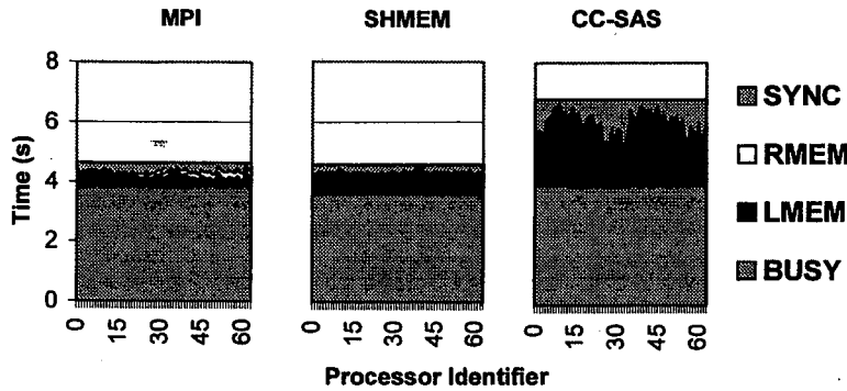
Figure 10: Time breakdown for the 1M data set on 64 processors.
