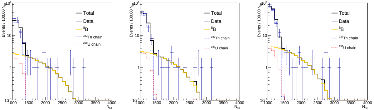
Figure 5.3: The best fit result plotted against the data for the partial fill ^8\text{B} flux analysis in the 4.5-m fiducial volume (left), the 5.0-m fiducial volume (center) and the 5.5-m fiducial volume (right).
