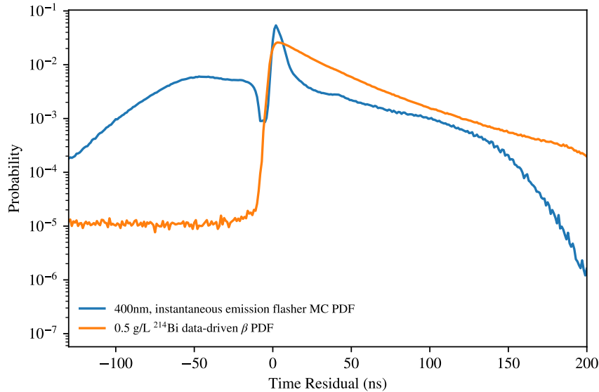
Figure 4.17: PDFs used for the flasher classifier analysis, normalized by area.
