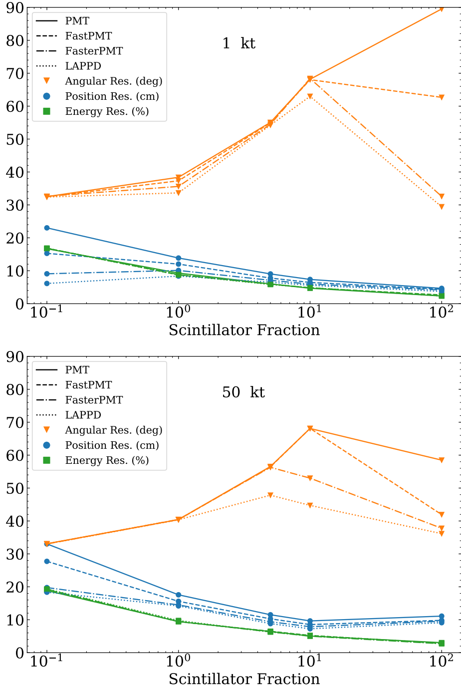
Figure 7.1: The achieved resolutions for position, direction and energy for the specified photodetector time response models and target materials, for the 1 kiloton and 50 kiloton scale detectors. Water is arbitrarily plotted with a scintillator fraction of 10^{-1} due to the axis's log scale.
