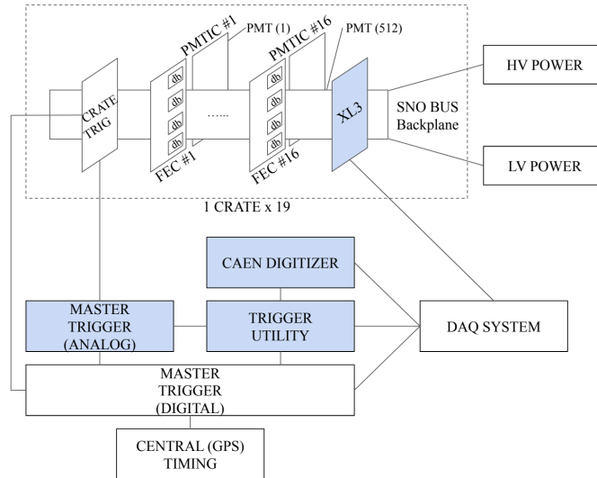
Figure 4.10: A schematic featuring the electronics readout chain for SNO+, with the upgrades from SNO featured in blue, as reproduced from [173].
