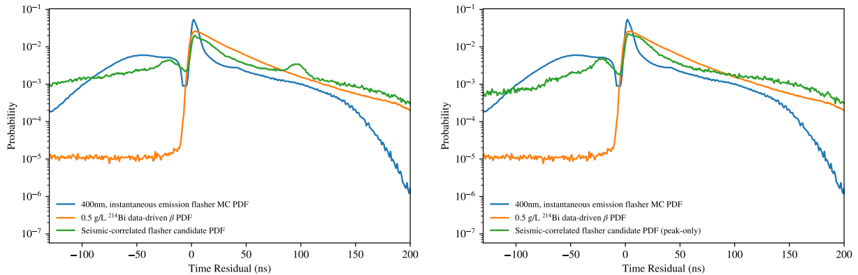
Figure 4.23: The extracted timing for flasher candidates in the seismic data compared with PDFs used for the flasher classifier analysis (left) with the extracted timing for flasher candidates in the seismic data restricted only to events in peak regions compared with PDFs used for the flasher classifier analysis (right). Normalization is by area for all curves in both plots.
