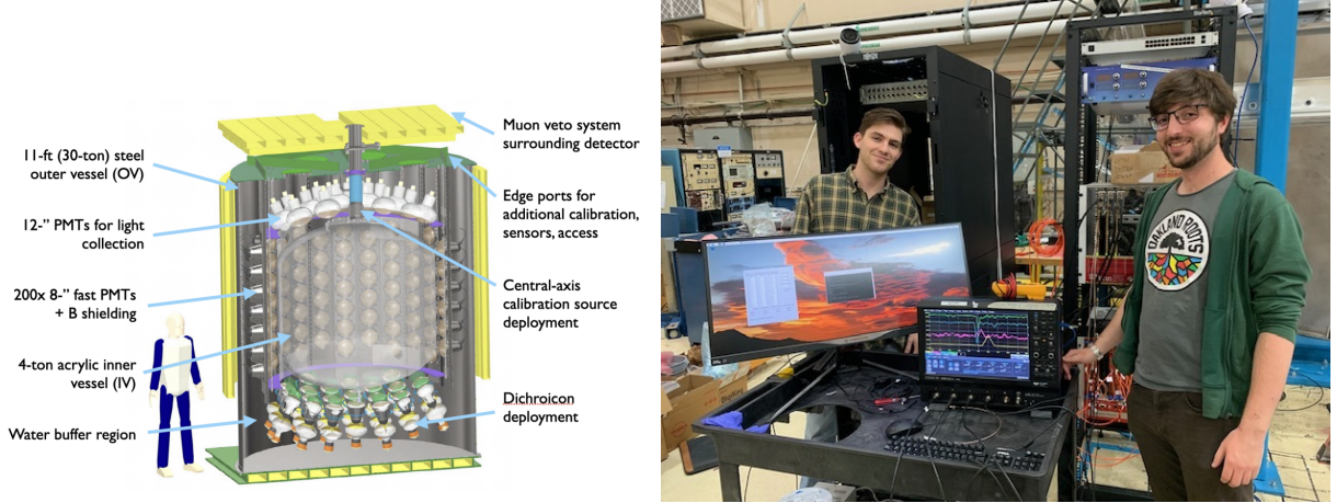
Figure 6.3: On left, a rendering of the EOS with various components labeled, reproduced from [114]. On right, the author (bespectacled) and collaborator B. Harris of the University of Pennsylvania show off the first PMT pulses read out from the EOS detector.
