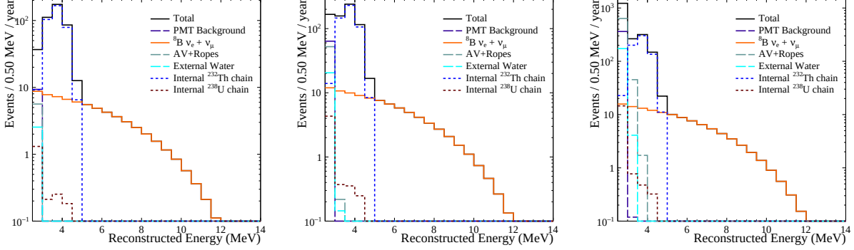
Figure 5.6: The PDFs in E for the full fill ^8\text{B} flux analysis scaled to a 780 t yr exposure for the 4.5-m fiducial volume (left), the 5.0-m fiducial volume (center) and the 5.5-m fiducial volume (right).
