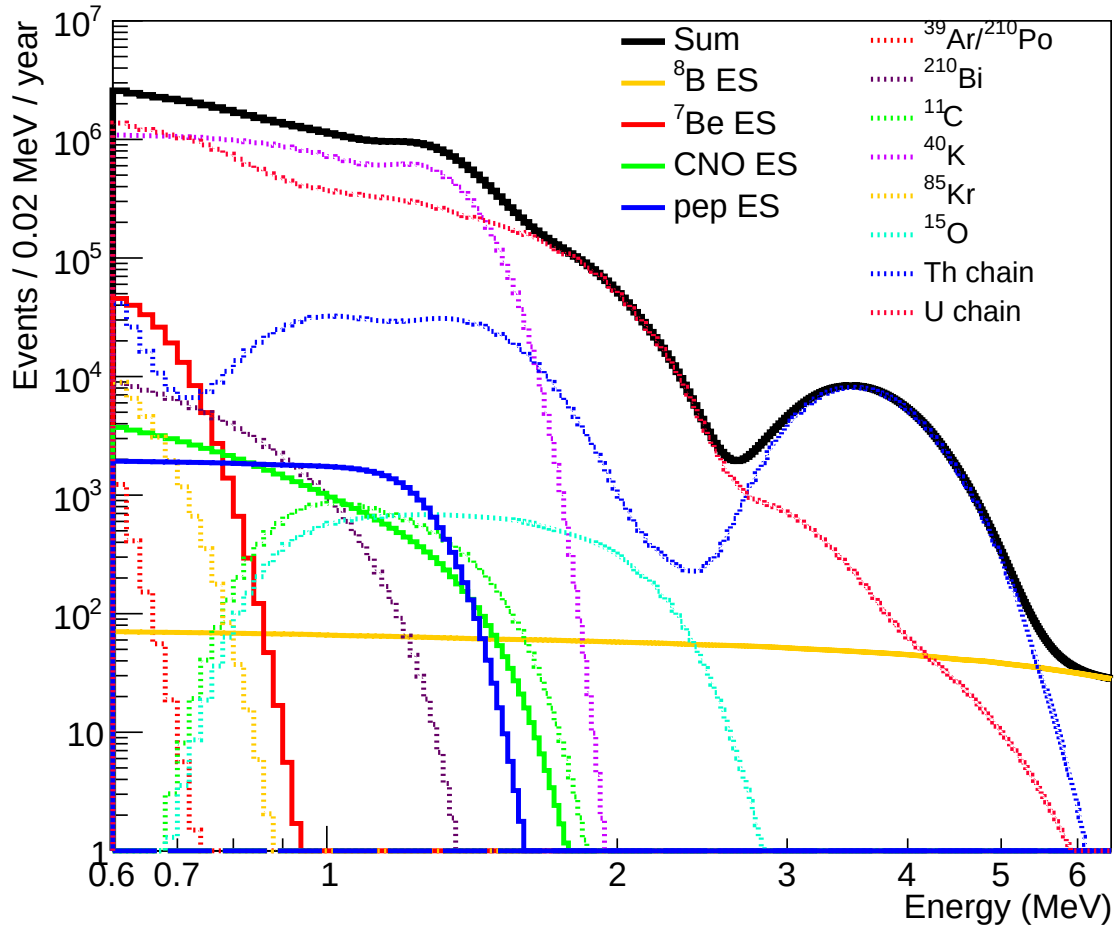
Figure 7.2: Energy spectrum from [1] for solar neutrino signals and radioactive backgrounds for a 25 kt, 5% WbLS detector, with 5 years of data-taking and using a simplified lookup-based reconstruction method for energy as discussed in [278].
