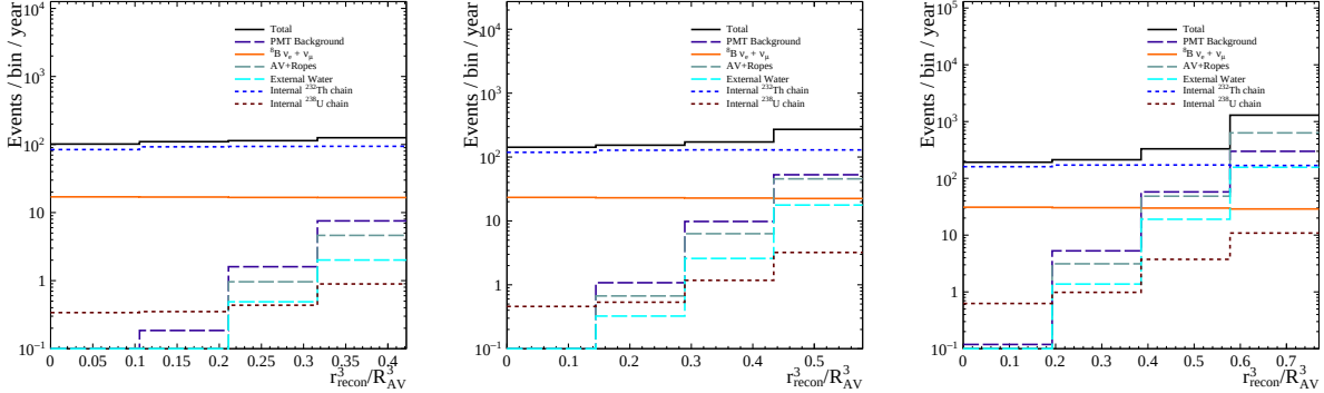
Figure 5.7: The PDFs in r^3/r_{\text{AV}}^3 for the full fill ^8\text{B} flux analysis scaled to a 780 t yr exposure for the 4.5-m fiducial volume (left), the 5.0-m fiducial volume (center) and the 5.5-m fiducial volume (right).
