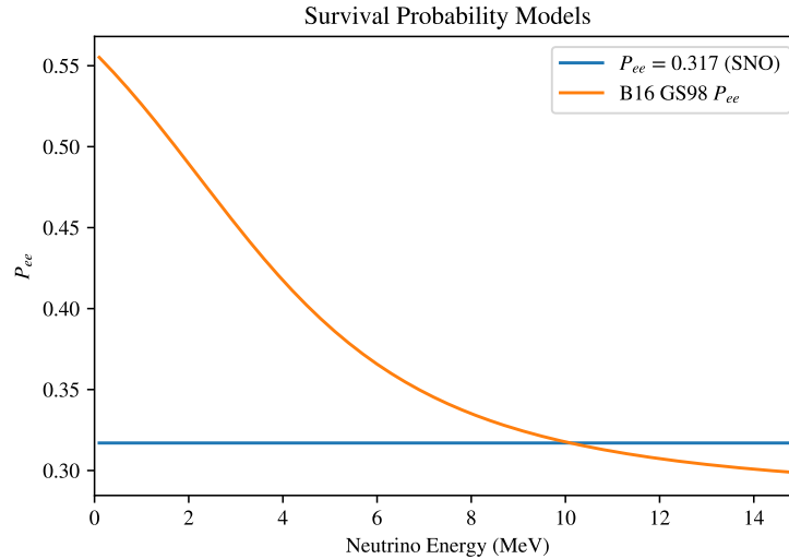
Figure 5.1: The survival probability P_{ee} as calculated in PSelmaa using the B16 GS98 Standard Solar Model and the PDG20 mixing parameters, as a function of neutrino energy. Also plotted is the best fit value for the flat contribution to the P_{ee} as measured by SNO [63].
