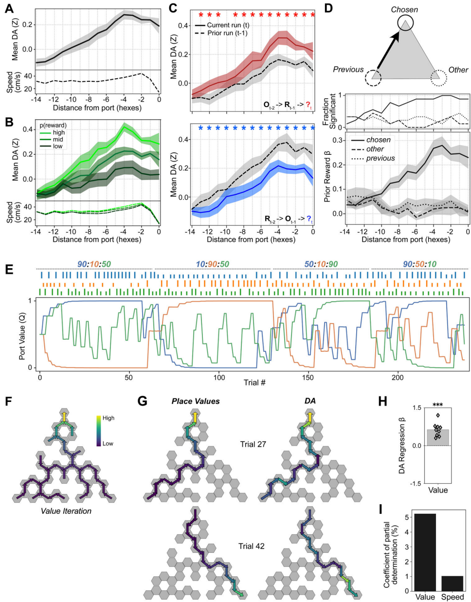
Fig. 3. DA ramps reflect dynamic expectations of upcoming reward. A , Mean hex-level running speed ( top ) and DA ( bottom ) as rats approached the reward ports (n = 10 rats, 82 sessions, 15918 trials), as a function of distance. B , Mean hex-level running speed ( top ) and DA ( bottom ) during port approach, pooled by p(reward) of the destination port. Only the second half (trial number > 25) of each block was included (n = 9 rats, 70 sessions, 7,614 trials). C , Examining the effects of reward on DA ramping along successive runs to the same port. Dashed lines indicate the prior run to the port (t-1), and solid lines indicate the current run to the port (t). Top , mean DA over successive runs to the same port, where reward was omitted two visits ago (t-2), but reward was delivered the prior visit (t-1; n=9 rats, 1935 sequences). Red asterisks indicate a significant increase in hex-level DA (p < 0.05, one-tailed Wilcoxon signed rank test). “R” and “O” denote
