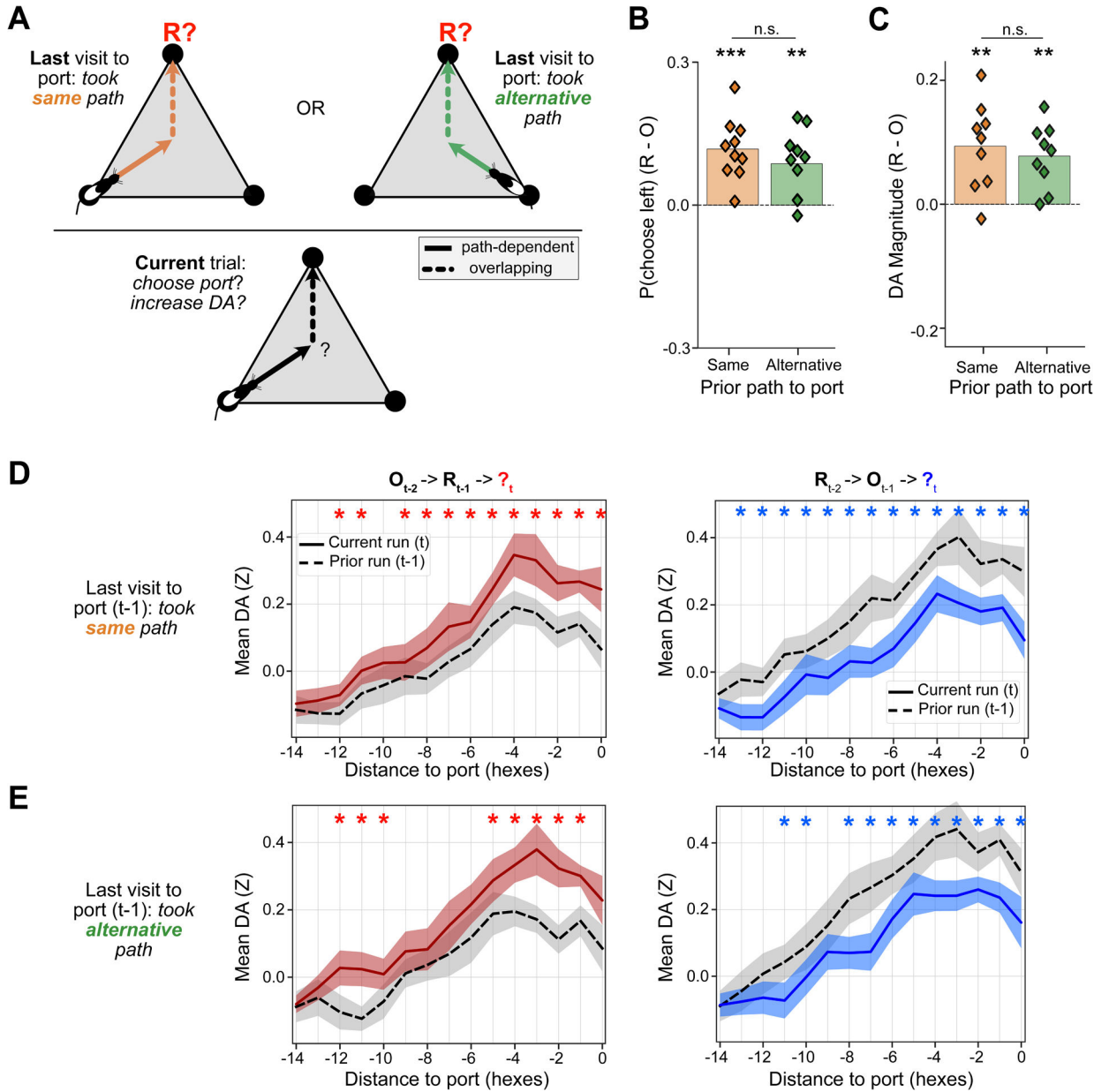
Fig. 5. Model-based inference globally updates DA place values and guides choices.
