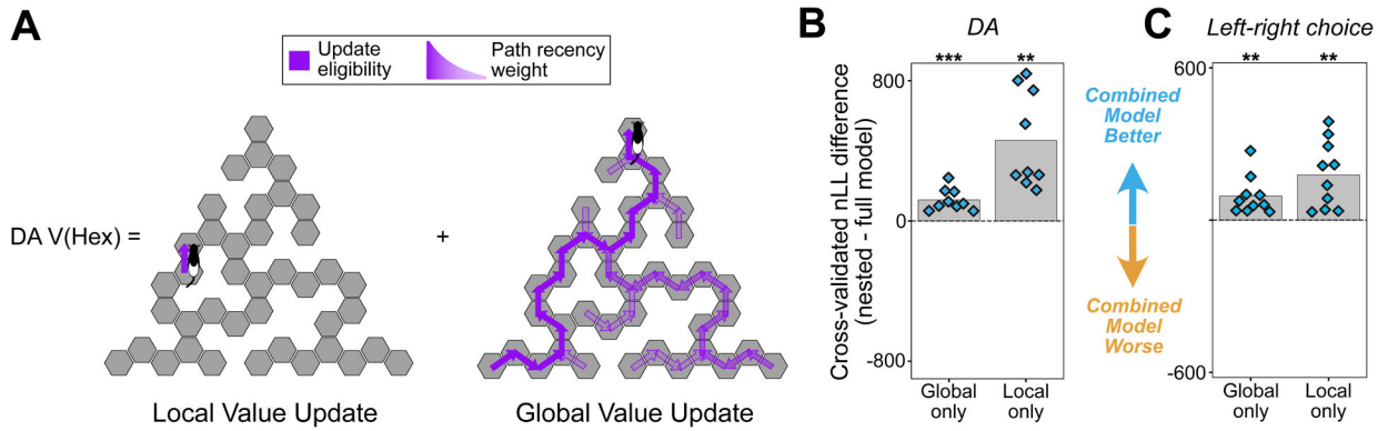
Fig. 6. A combined local and global value-update model accounts for hex-level DA.
