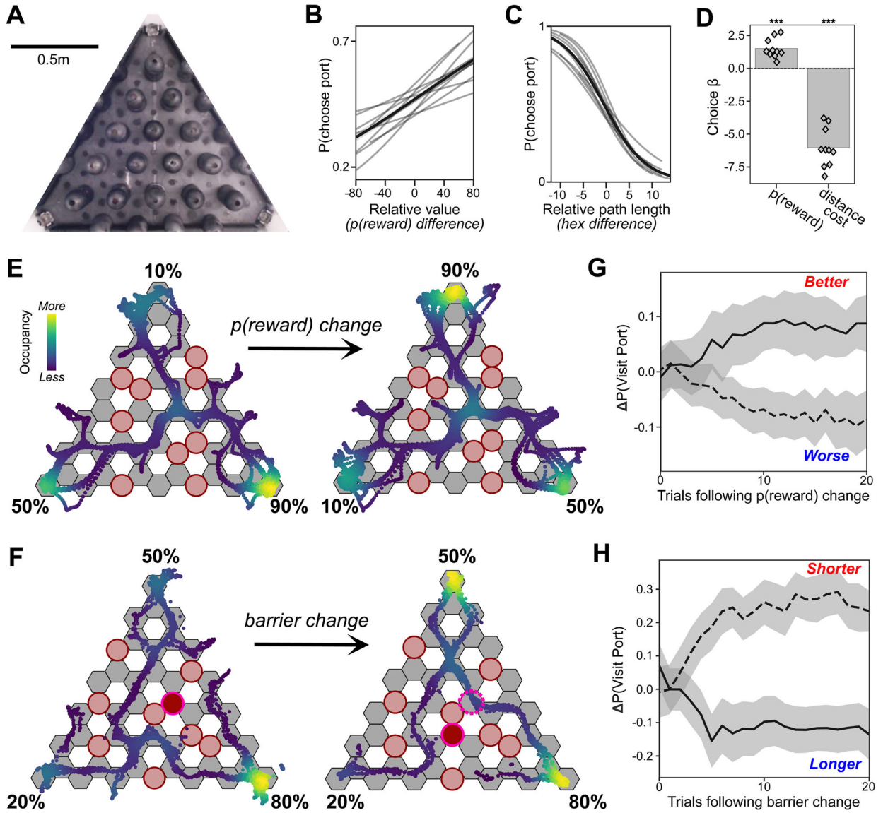
Fig. 1. Adaptive behavior in the spatial foraging task.
