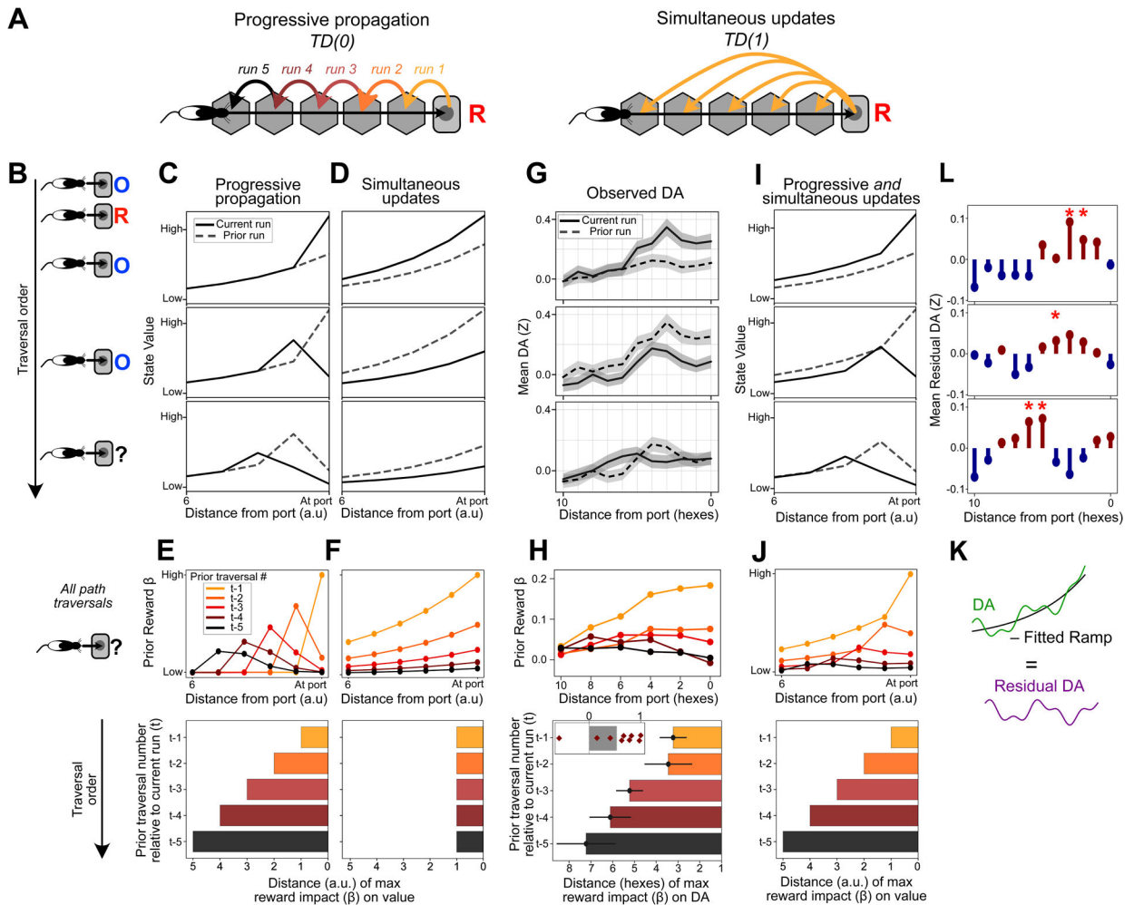
Figure 4. Progressive propagation of DA signals across space.
