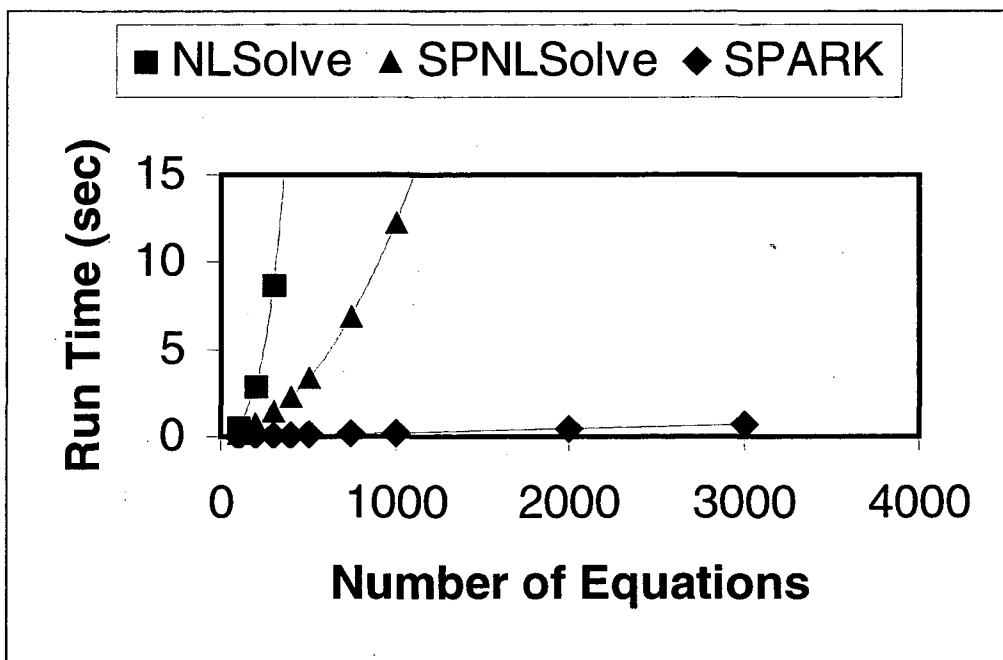
Figure 1: Solution times for nonlinear benchmark, SPARK vs., Meschach.
