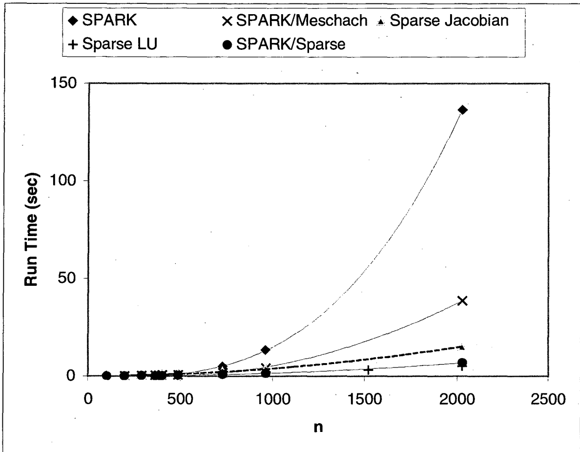
Figure 3: Solution times for the Laplace's equation example.
