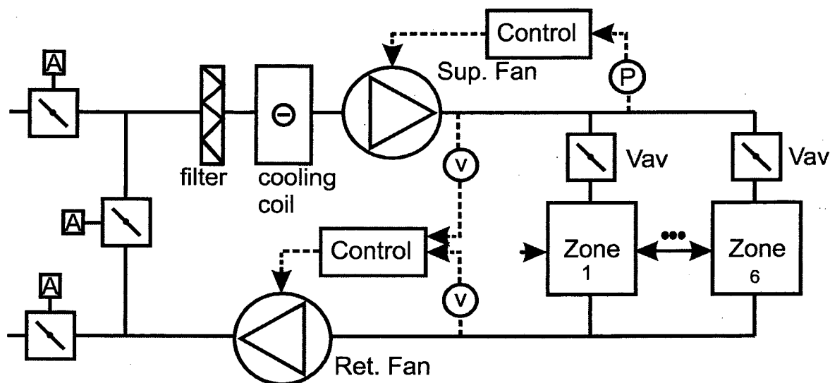
Figure 4 HVAC system.
