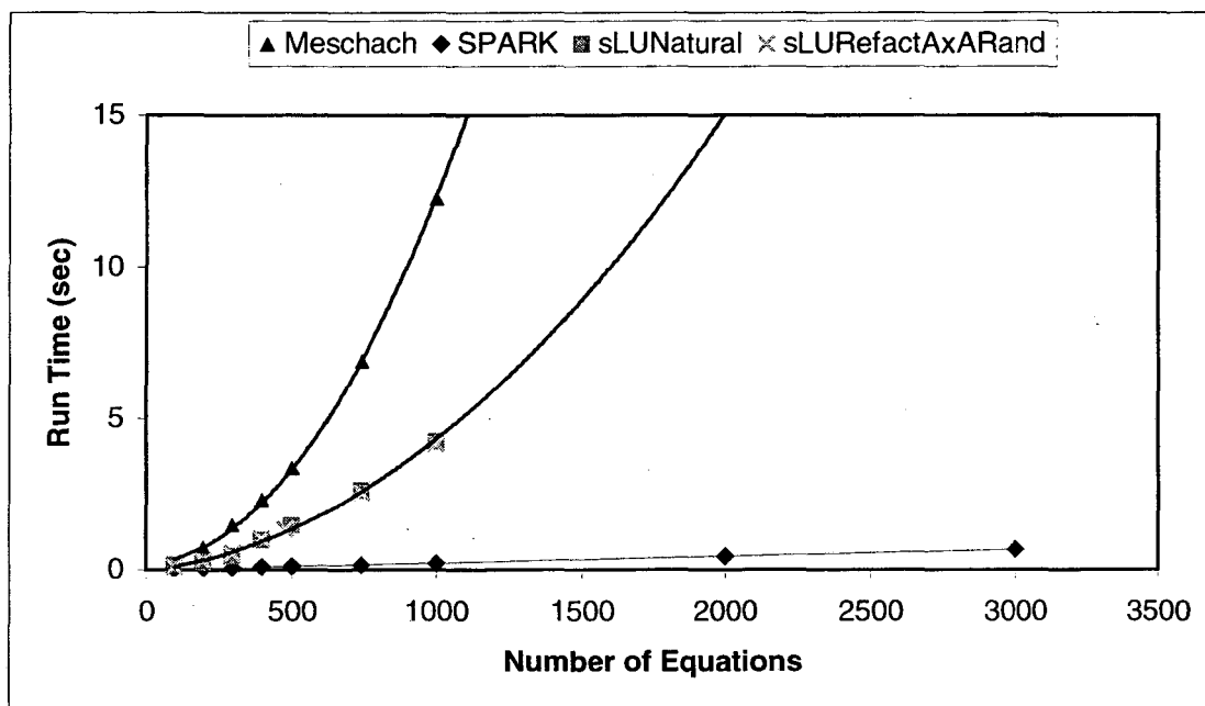
Figure 2: Solution times for nonlinear benchmark, SPARK Vs, SuperLU.
