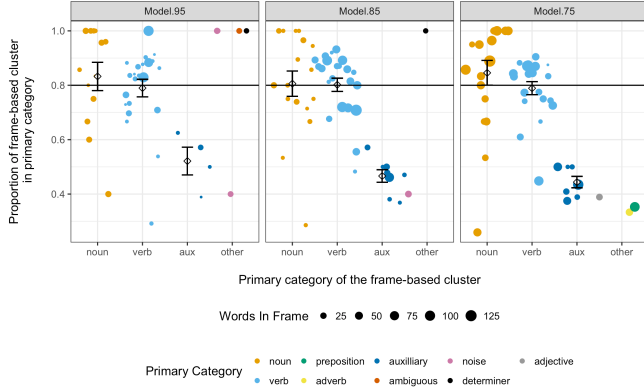
Figure 1b: Accuracies of the 50 most frequent frames in the within-word corpus. The horizontal line indicates 80% accuracy. Point size represents number of words per frame.
