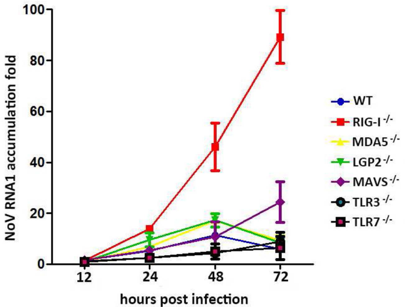
Figure 1. RIG-I deficiency leads to increased NoV replication in MEFs Mouse embryo fibroblasts from wild type (WT), RIG-I -/- , MDA5 -/- , LGP2 -/- , MAVS -/- , TLR3 -/- and TLR7 -/- were inoculated with NoV at amount of viral genome copies ( 5 \times 10^6 ). RNA1 levels of NoV were determined at 12, 24, 48 and 72 hpi for each sample by real-time RT-PCR.
