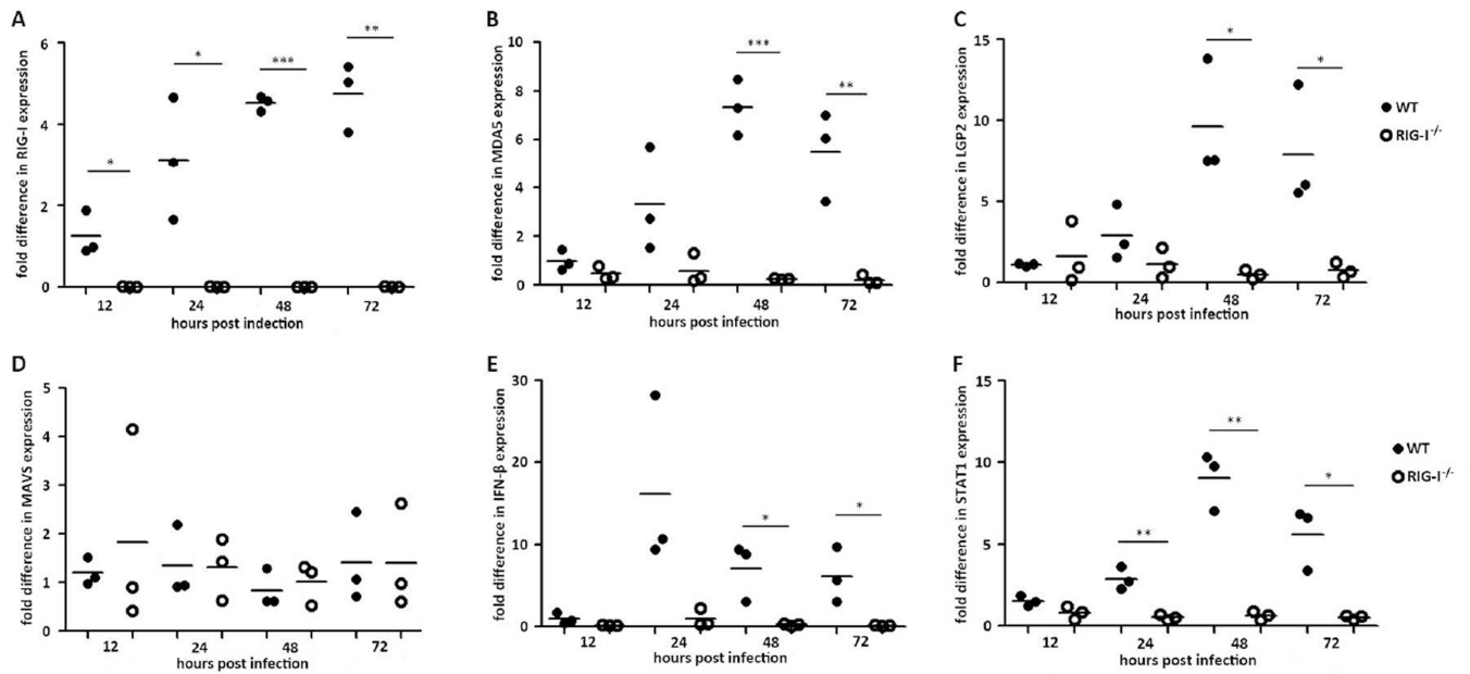
Figure 2. Expression profiles of innate immune-related genes in RIG-I -/- MEFs WT and RIG-I -/- MEFs were infected with NoV for 12, 24, 48 and 72hpi. Cells of each sample were harvested and total RNA extracted. RIG-I (A), MDA5 (B), LGP2 (C), MAVS (D), IFN-β (E) and STAT1 (F) mRNA levels were determined by real-time RT-PCR and normalized by mRNA levels expressed in mock-inoculated MEFs.
