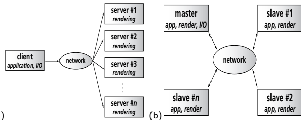
Figure 6: Cluster rendering distribution schemes: (a) client-server, (b) master-slave.
