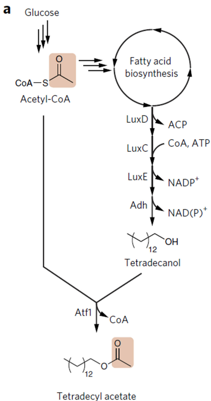
Figure 3. Tetradecyl acetate production from glucose in E. coli
