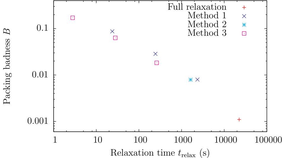
Fig. 12. Logarithmic plot of the packing badness B versus the total time spent on relaxation in the simulation t_{\text{relax}} , for the simulation with full relaxation, and the simulations with the three different types of infrequent relaxation.
