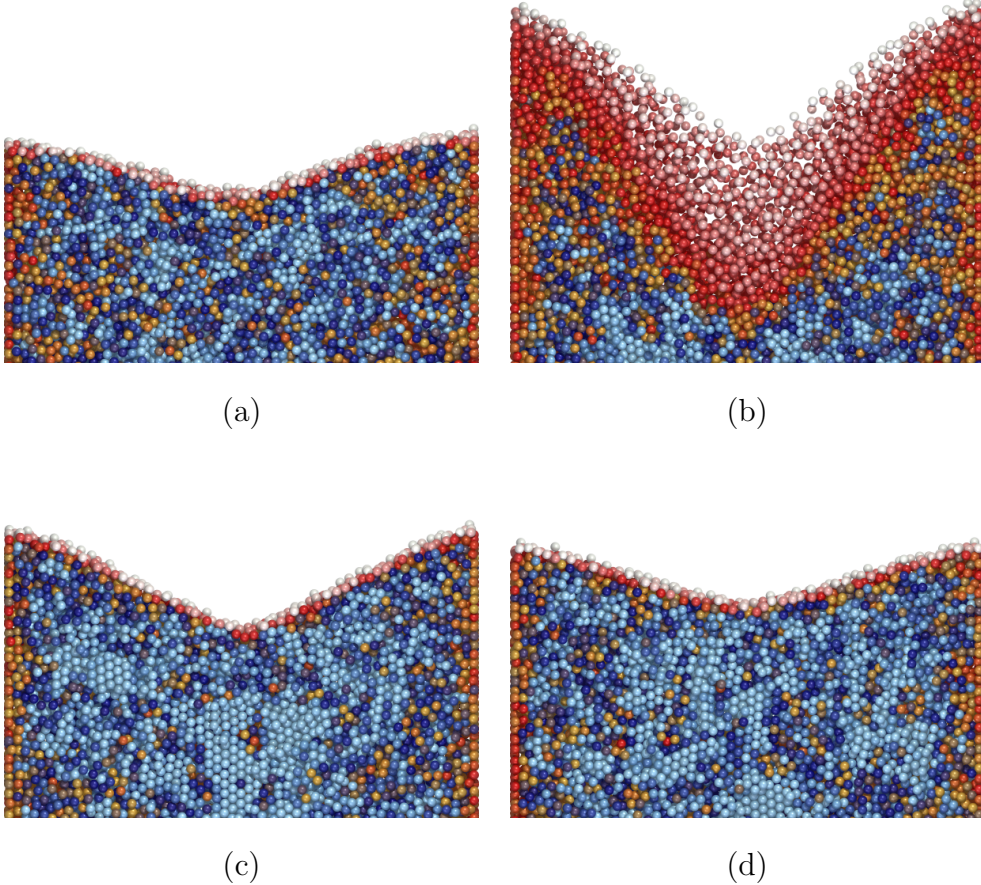
Fig. 6. Close-up snapshots of the free surface of the particle packings for the same simulations in figure 5, for the region 50d < z < 90d . Each particle is colored according to its local packing fraction, computed as the ratio of its volume to its Voronoi cell volume. The central slice of the packing is shown by only plotting particles with y > 0 . The same color scheme is used as for figure 4.
