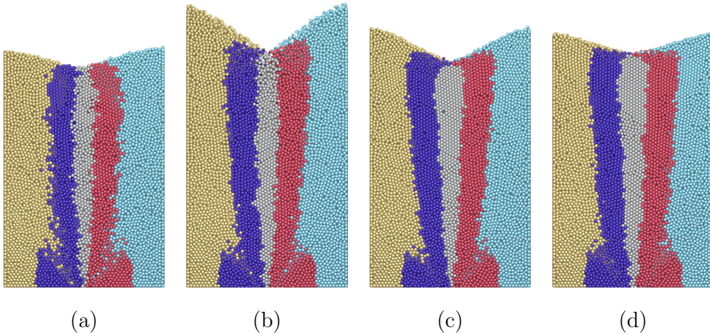
Fig. 5. Snapshots of (a) DEM simulation, (b) a spot simulation using a random walk with simple biasing, (c) a spot simulation using simple biasing and influence weighting, and (d) a spot simulation using adapted biasing (with \beta = 3 ) and influence weighting. The snapshots are taken at t = 300\tau .
