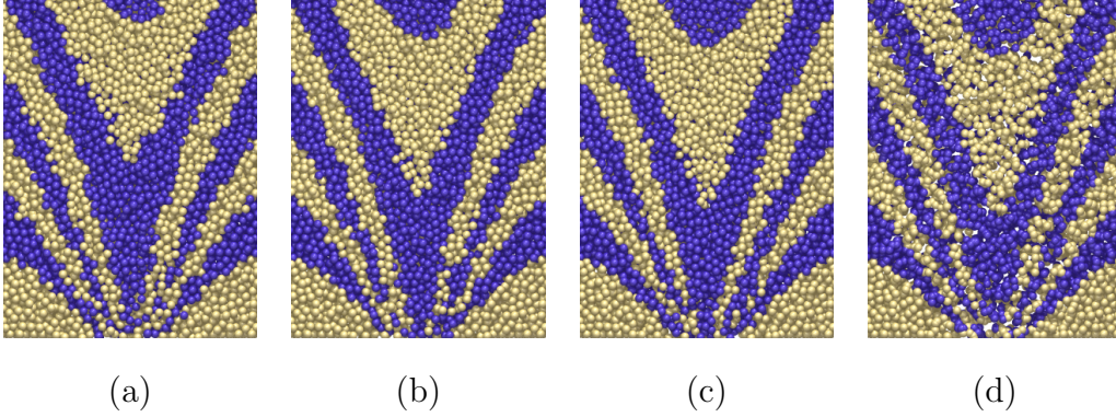
Fig. 10. Snapshots at t = 120\tau for (a) the original simulation, (b) the method 1 simulation with k = 100 , (c) the method 1 simulation with k = 1000 , and (d) the simulation with no relaxation. The region -15d < x < 15d, 0 < z < 40d is shown, and only particles with y > 0 are plotted, to view the central slice of the particle packings.
