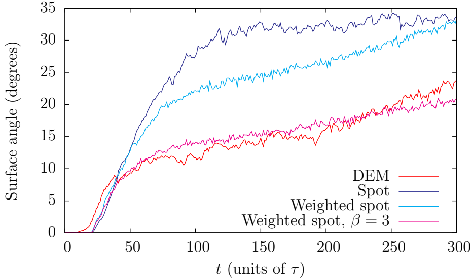
Fig. 7. Time evolution of the angle of the free surface, calculated using linear regression, of the four simulations shown in figure 5.
