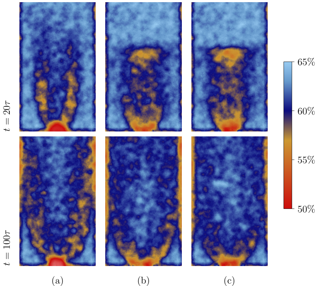
Fig. 4. Plots of local packing fraction at two different times, for (a) the DEM simulation, (b) the event-driven spot simulation, and (c) the fixed timestep spot simulation. At each point, the local packing fraction is computed by finding all particles within a distance of 2.2d of that point, and then dividing the total particle volume by the total volume of their Voronoi cells. (For packing fractions in the range 0%–50% near the orifice, the color is smoothly graded from white to red.)
