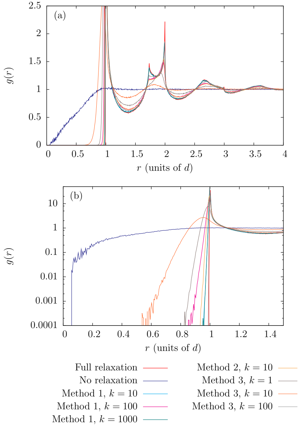
Fig. 11. The radial distribution function g(r) for the spot simulations listed in figure 9, computed in a central region of flow, -15d < x < 15d, 15d < z < 45d for all snapshots over the range 40\tau \leq t \leq 200\tau . Part (a) shows the complete curves for the range 0 < r < 4d , while part (b) shows a semi-logarithmic plot of the region 0 < r < 1.5d , to highlight the part of the distributions that correspond to overlapped particles.
