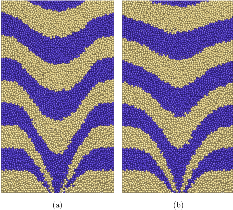
Fig. 3. Snapshots of the (a) DEM simulation and (b) event-driven spot simulations at t = 60\tau . The central slice of the packing is shown, by only plotting those particles with y > 0 . The two colors of particles are physically identical and initially form layers of thickness 10d , and are used to highlight the flow and particle mixing that takes place.
