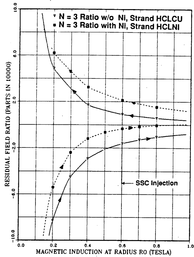
Fig. 6 A comparison of the magnetization sextupole ratio at R=1 cm versus central induction for a SSC dipole with HLCU and HCLNI strands
