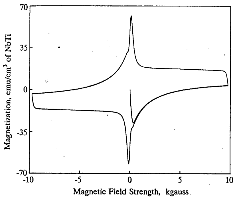
Fig. 3 Magnetic hysteresis loop for strand HCLNI at 4.2K.
