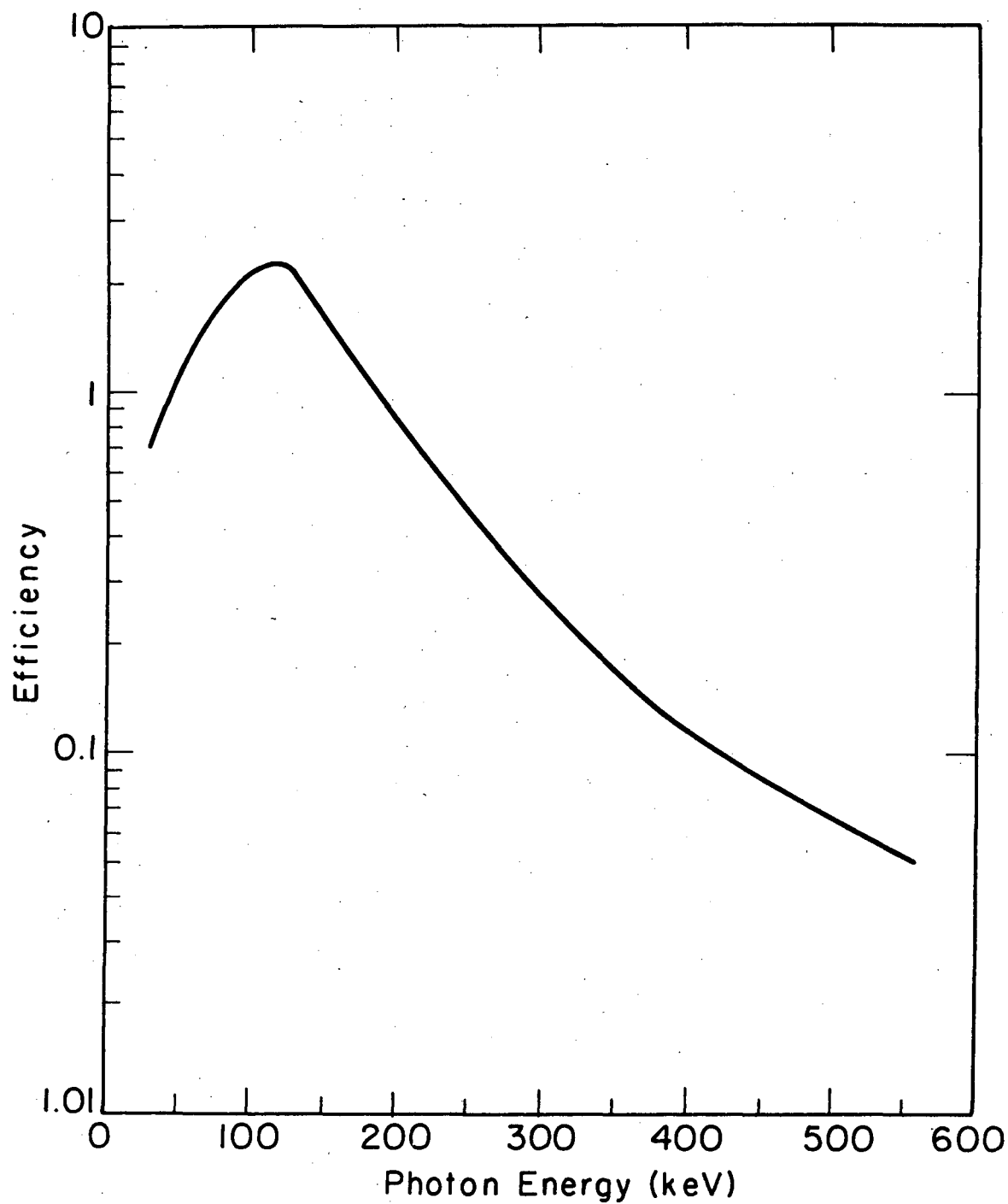
Fig. 15. Ge(Li) planar detector efficiency--arbitrary scale--versus photon energy. The efficiency curve takes also into account the geometrical configuration of the target-detector system.
