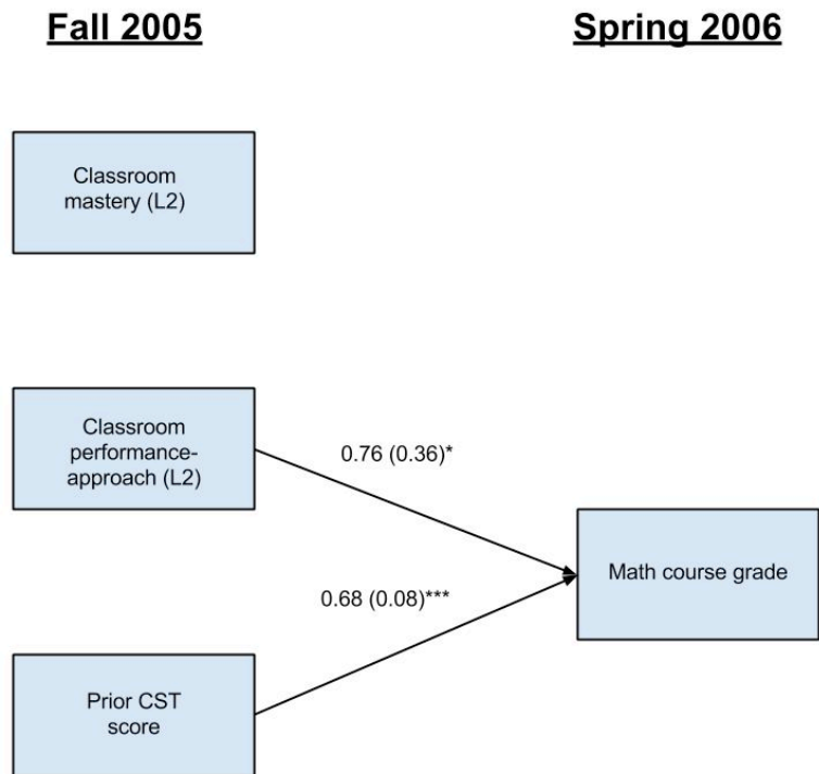
Figure 3.5. Multigroup SEM results for mastery goals perspective (a) and revised goals perspective (b) profile groups when structural parameters were allowed to be freely estimated between the two groups (Profiles 1 and 4, respectively). Statistically significant ( p < .05 ) unstandardized regression coefficients and covariances are reported.
