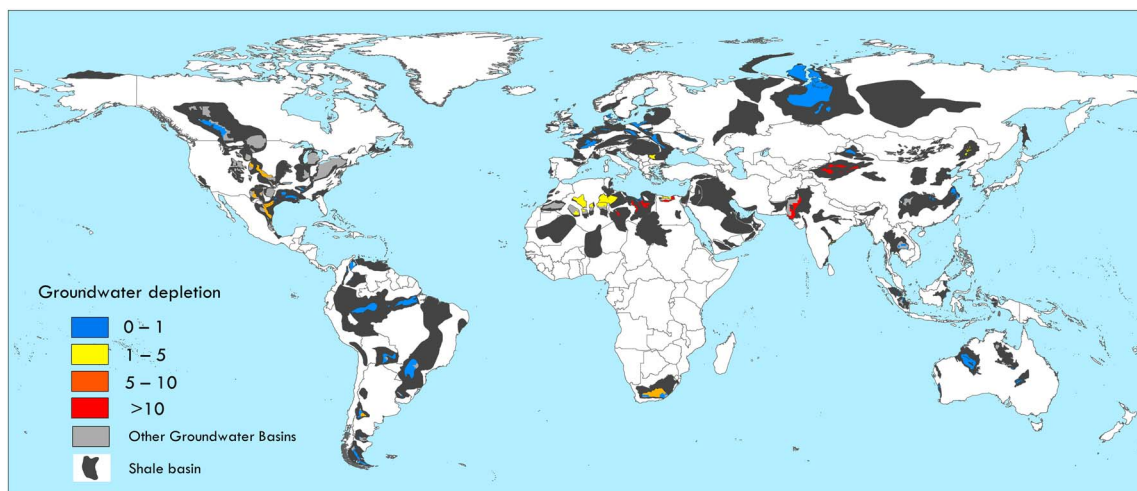
Figure 3. Groundwater-depleted aquifers in the footprint of world shale deposits. Freshwater aquifers considered are major groundwater basins (Gleeson et al, 2012). Pixels with groundwater depletion indexes greater than one indicate unsustainable water withdrawals (i.e., groundwater depletion).
