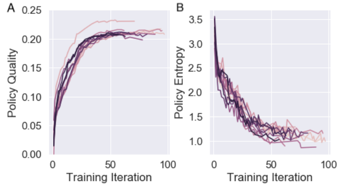
Figure 2: Policy quality and policy entropy. A) Policy quality of AlphaZero agents increases with training. B) Policy entropy of AlphaZero agents decreases with training
