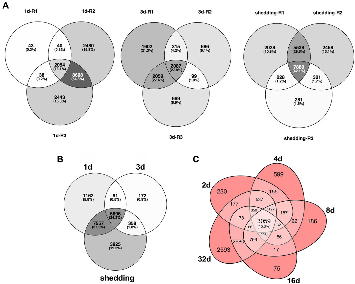
Fig 2. (A) Venn diagrams of S. mansoni replicates from Illumina sample groups. (B) Venn diagram of S. mansoni transcripts with \geq 1 \text{Log}_2(\text{TPM}) in at least one replicate per group. (C) Venn diagram of expressed unique S. mansoni probes with > 1 \text{Log}_2 fluorescence in the microarray.
