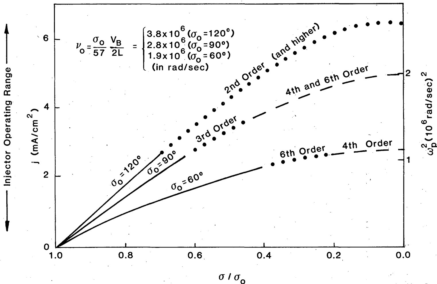
Fig. 8 Beam current density vs. space-charge depressed phase advance showing expected regions of instability. The definitions of the symbols and their interrelationships is given in the text.
