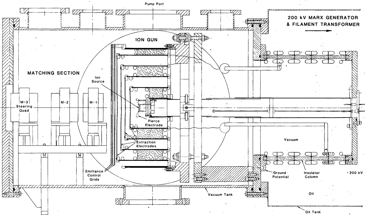
SINGLE BEAM TRANSPORT EXPERIMENT GUN & MATCHING SECTION
